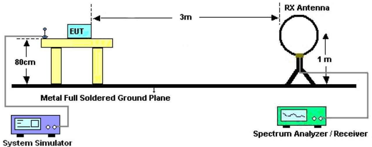
Figure 1. Below 30MHz
