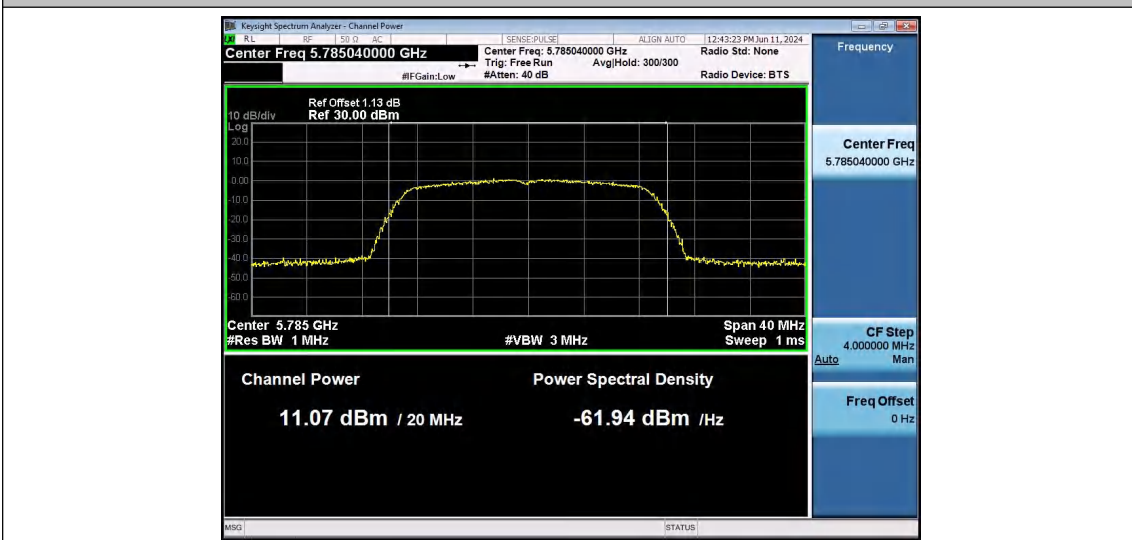
11AC20SISO-Ant1-5785-PASS
