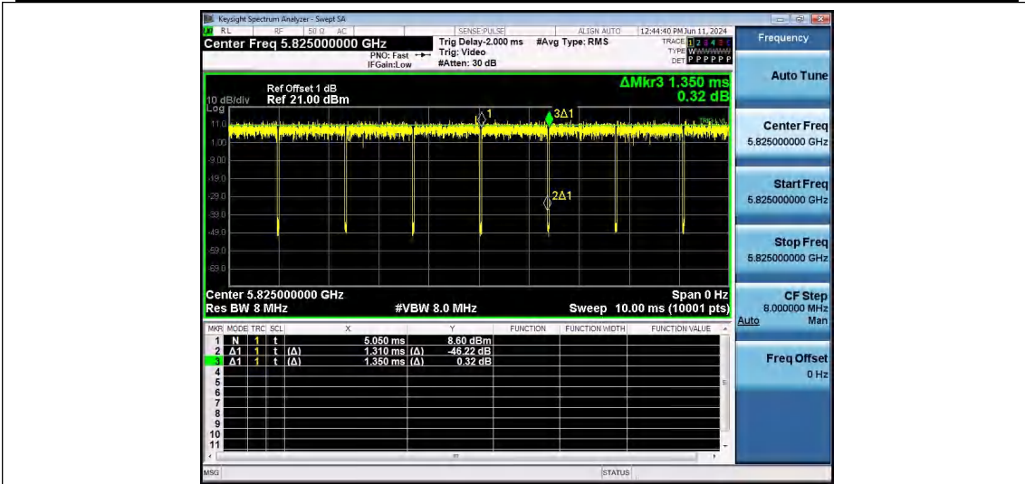
NTV-11AC20SISO-Ant1-5825
