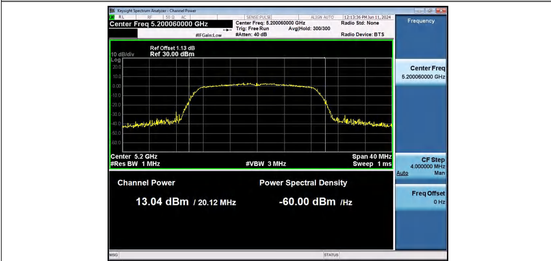
11AC20SISO-Ant1-5200-PASS
