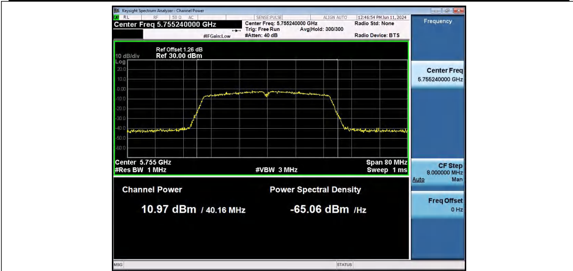
11AC40SISO-Ant1-5755-PASS
