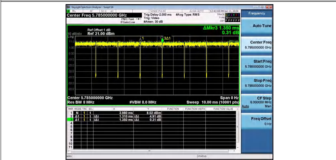
NTNV-11AC20SISO-Ant1-5785
