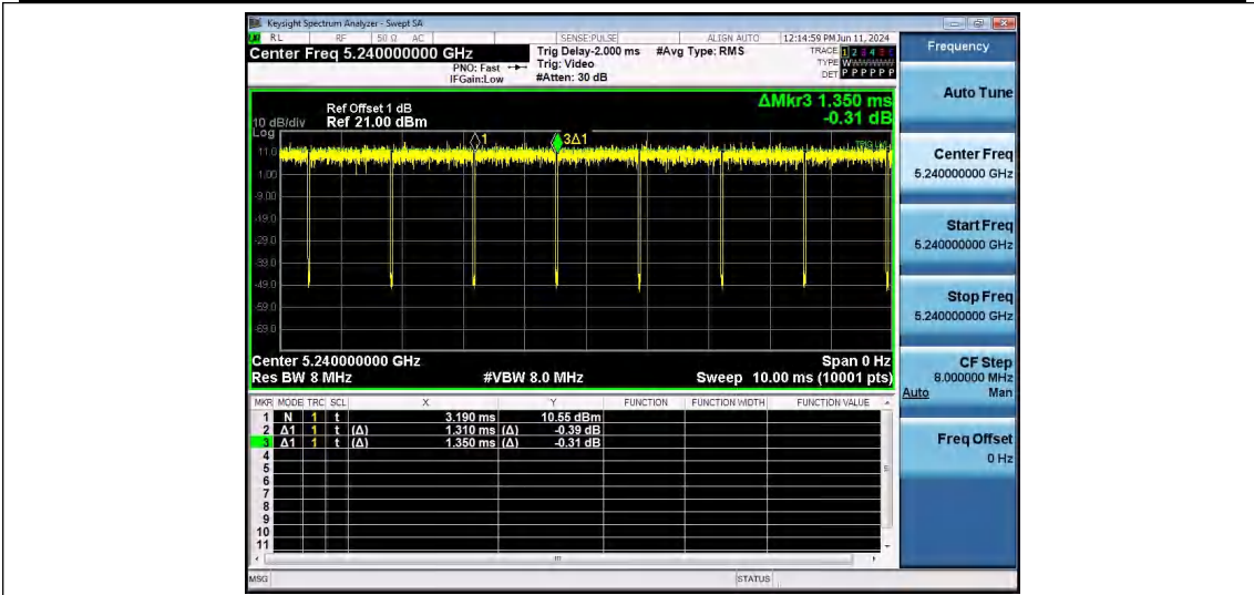
NTNV-11AC20SISO-Ant1-5240
