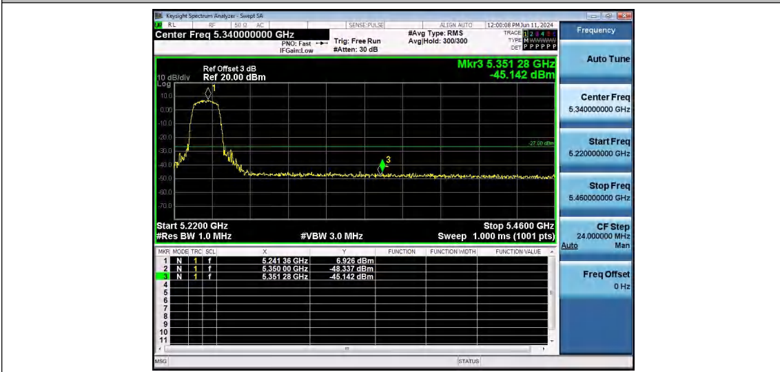
11A-Ant1-5240-PASS
