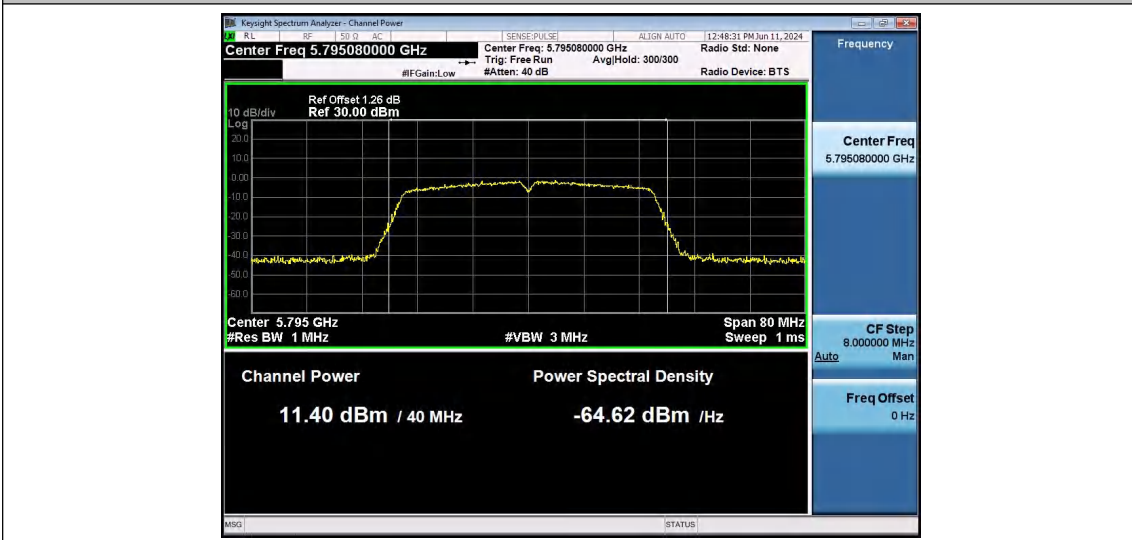
11AC40SISO-Ant1-5795-PASS
