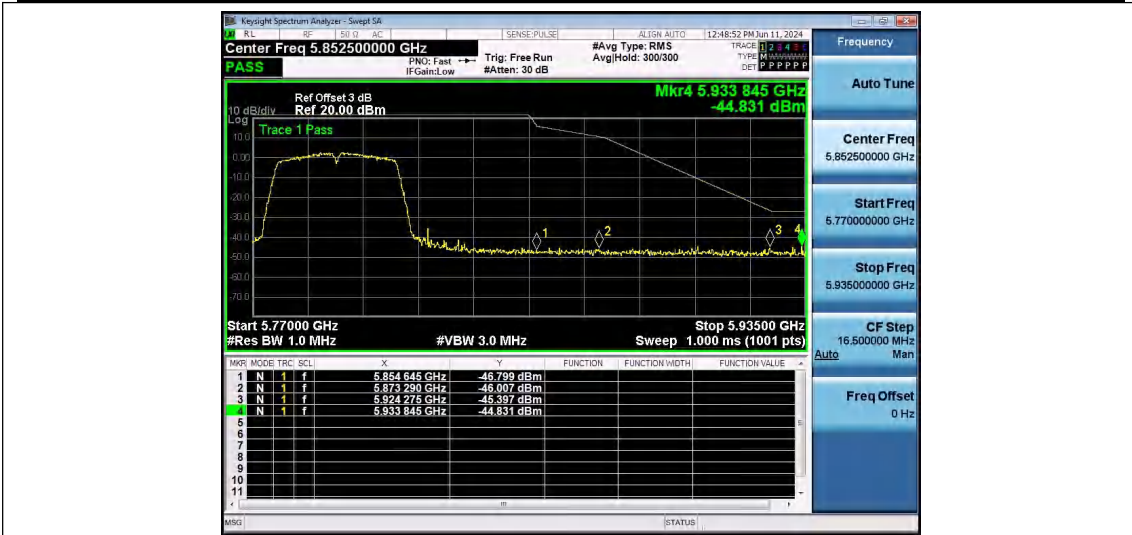
11AC40SISO-Ant1-5795-PASS
