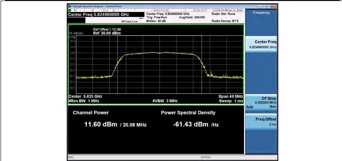
11AC20SISO-Ant1-5825-PASS
