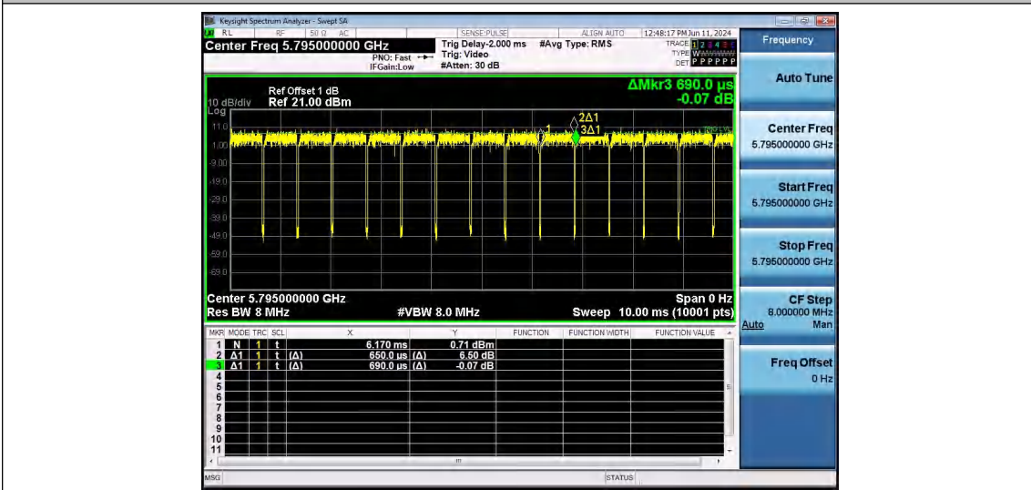
NTNV-11AC40SISO-Ant1-5795
