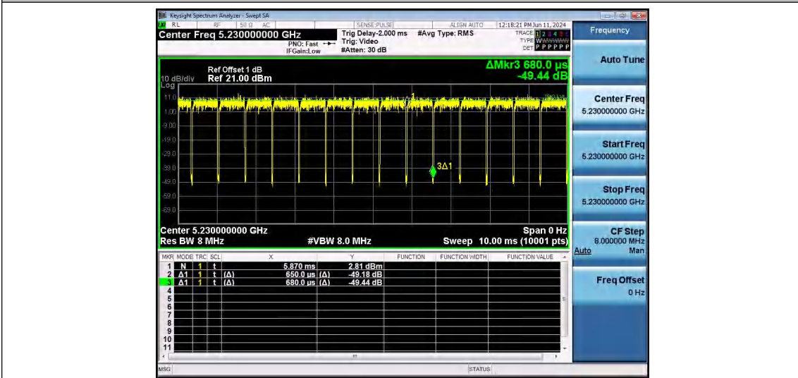
NTV-11AC40SISO-Ant1-5230
