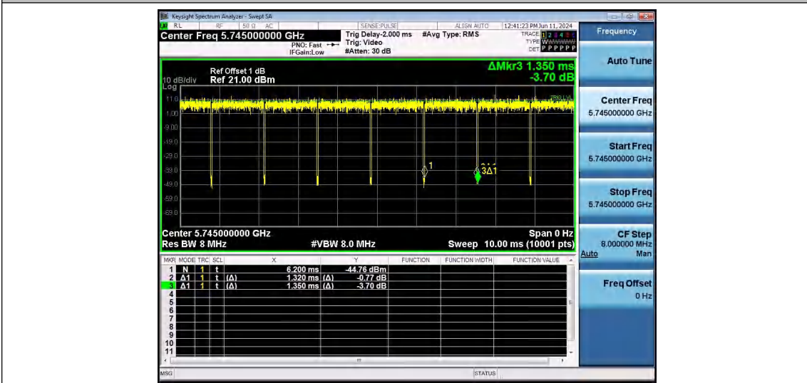
NTNV-11AC20SISO-Ant1-5745
