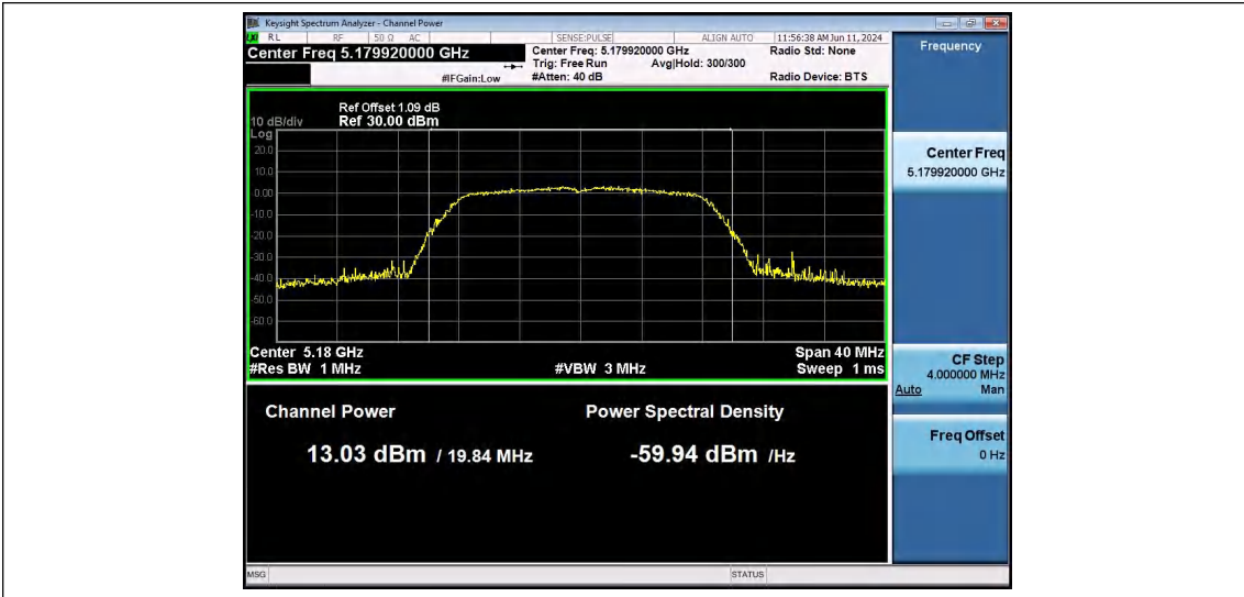
11A-Ant1-5180-PASS
