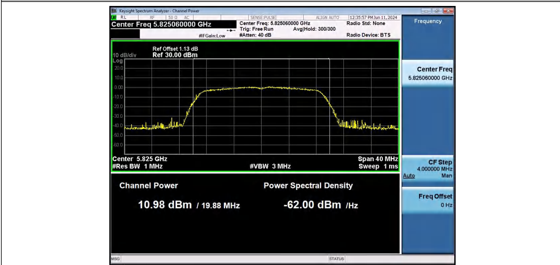
11N20SISO-Ant1-5825-PASS
