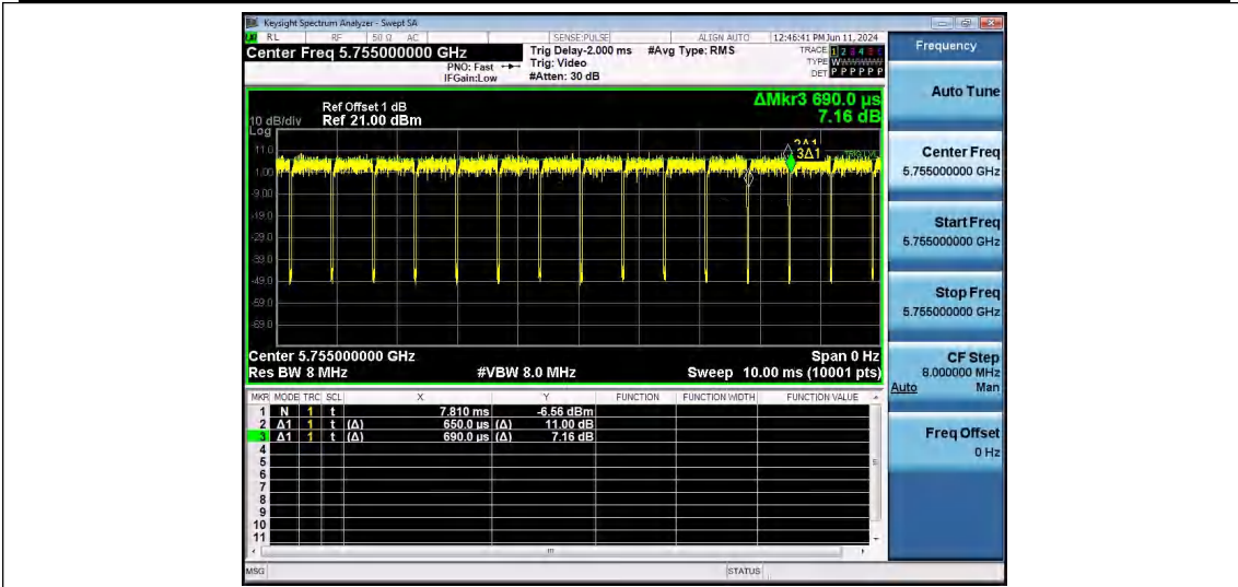
NTNV-11AC40SISO-Ant1-5755
