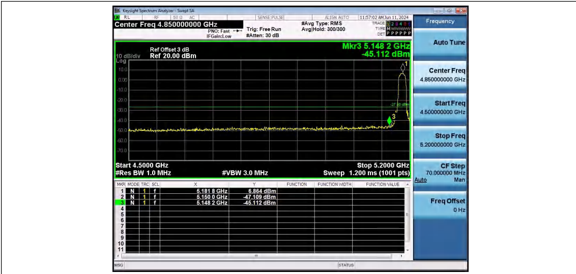
11A-Ant1-5180-PASS
