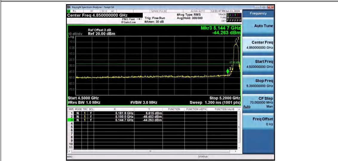
11N20SISO-Ant1-5180-PASS
