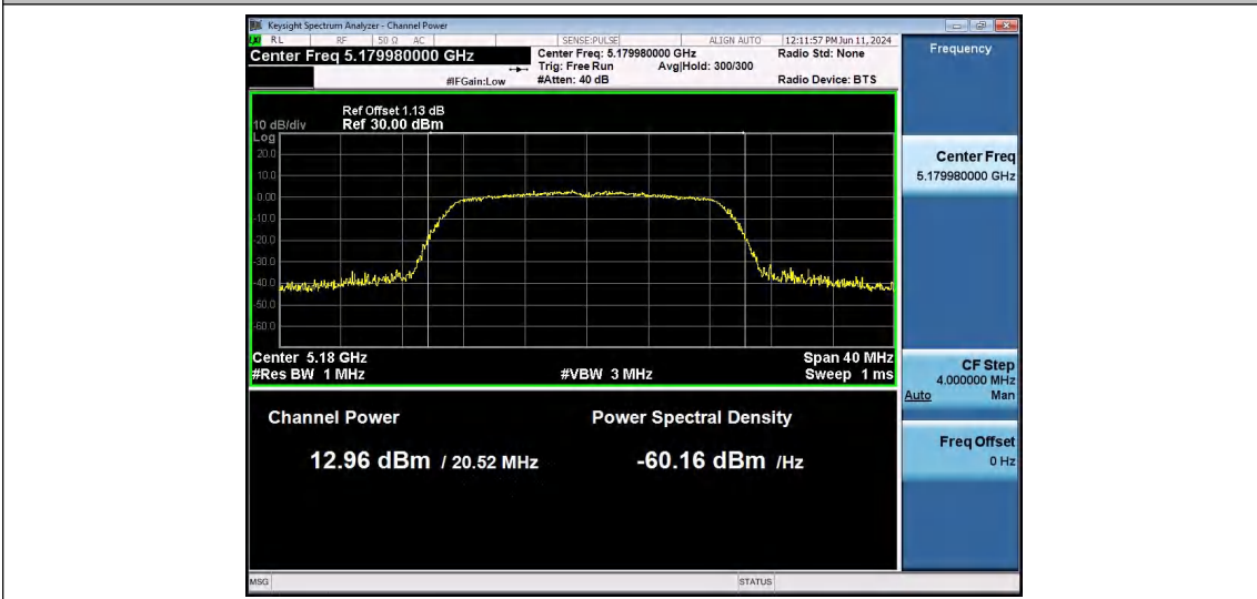
11AC20SISO-Ant1-5180-PASS
