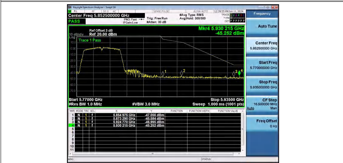
11N40SISO-Ant1-5795-PASS
