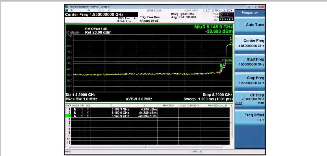
11N40SISO-Ant1-5190-PASS
