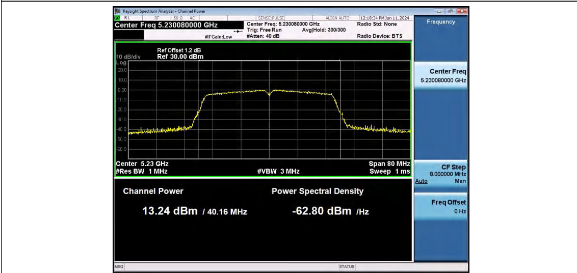
11AC40SISO-Ant1-5230-PASS
