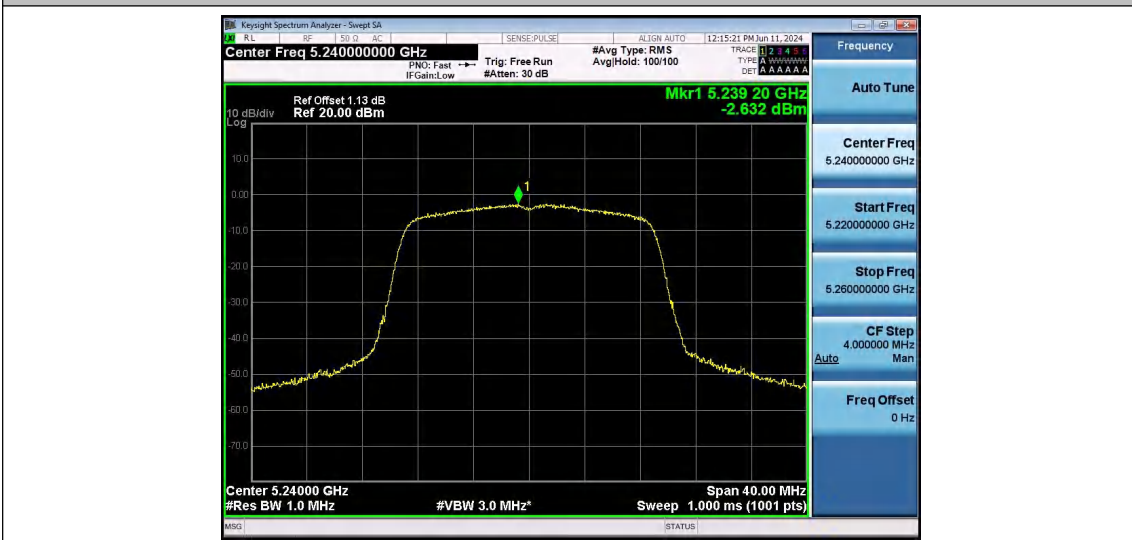
11AC20SISO-Ant1-5240-PASS
