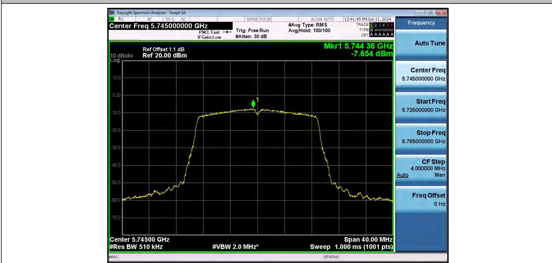
11AC20SISO-Ant1-5745-PASS
