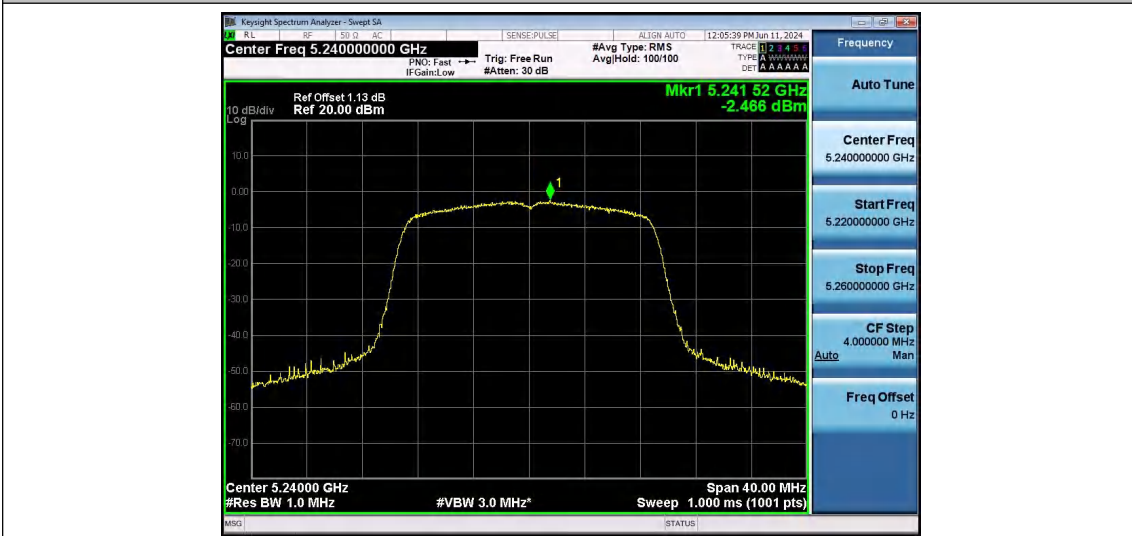
11N20SISO-Ant1-5240-PASS
