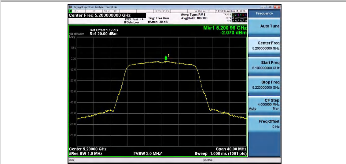
11A-Ant1-5200-PASS
