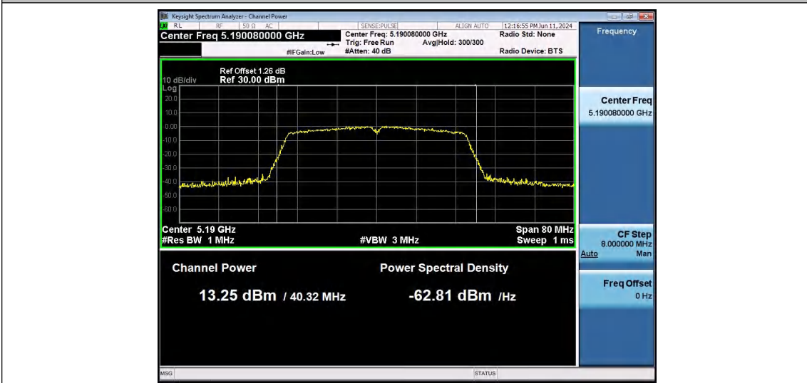
11AC40SISO-Ant1-5190-PASS
