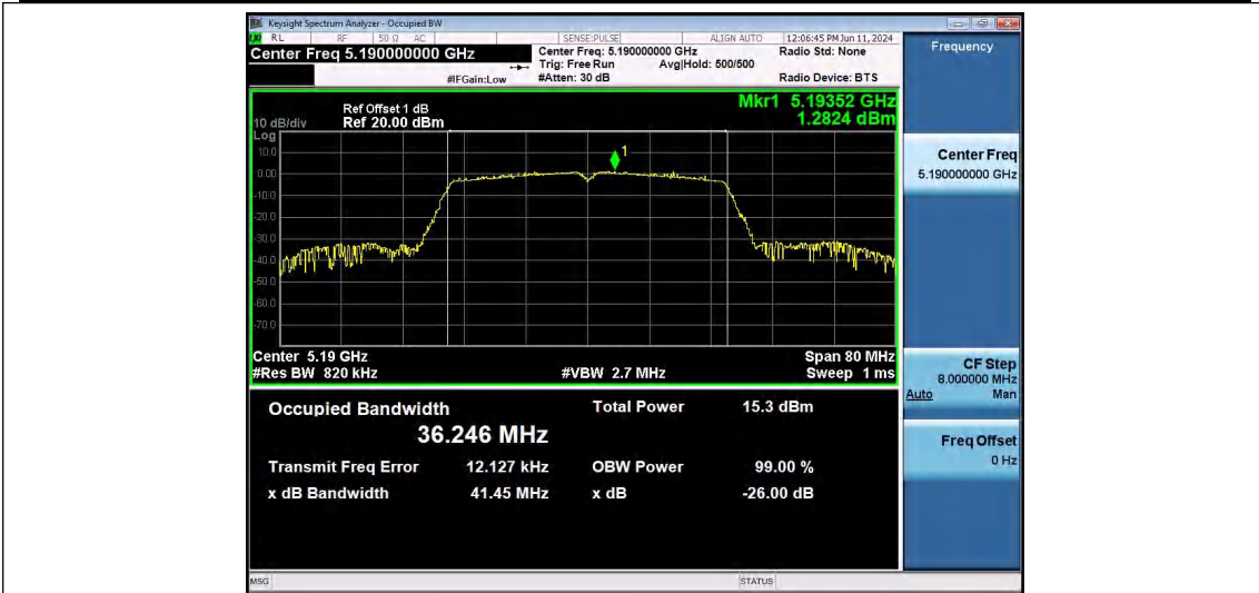
11N40SISO-Ant1-5190
