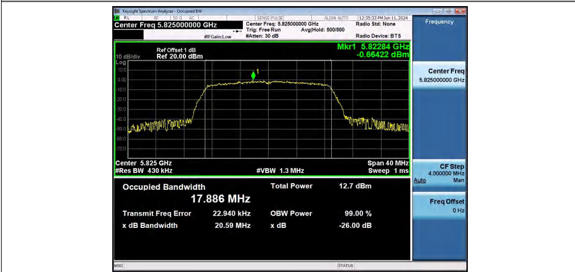
11N20SISO-Ant1-5825
