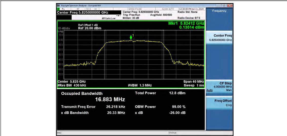
11A-Ant1-5825
