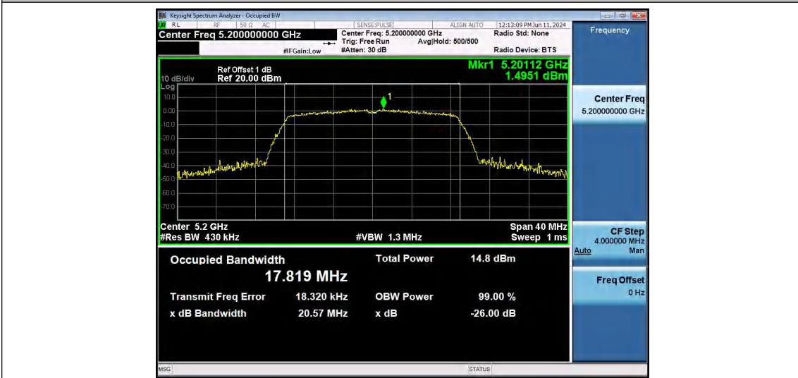
11AC20SISO-Ant1-5200
