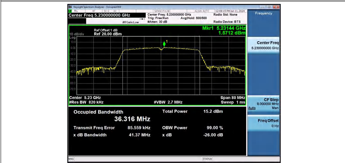
11N40SISO-Ant1-5230
