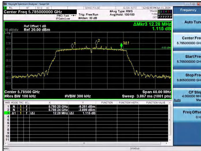
11AC20SISO-Ant1-5785-PASS
