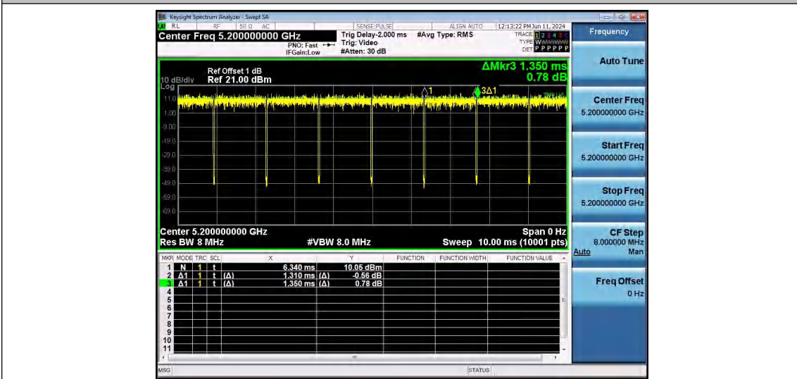
NTNV-11AC20SISO-Ant1-5200
