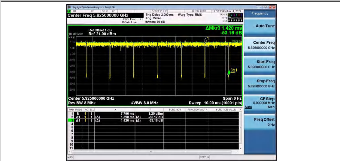
NTNV-11A-Ant1-5825
