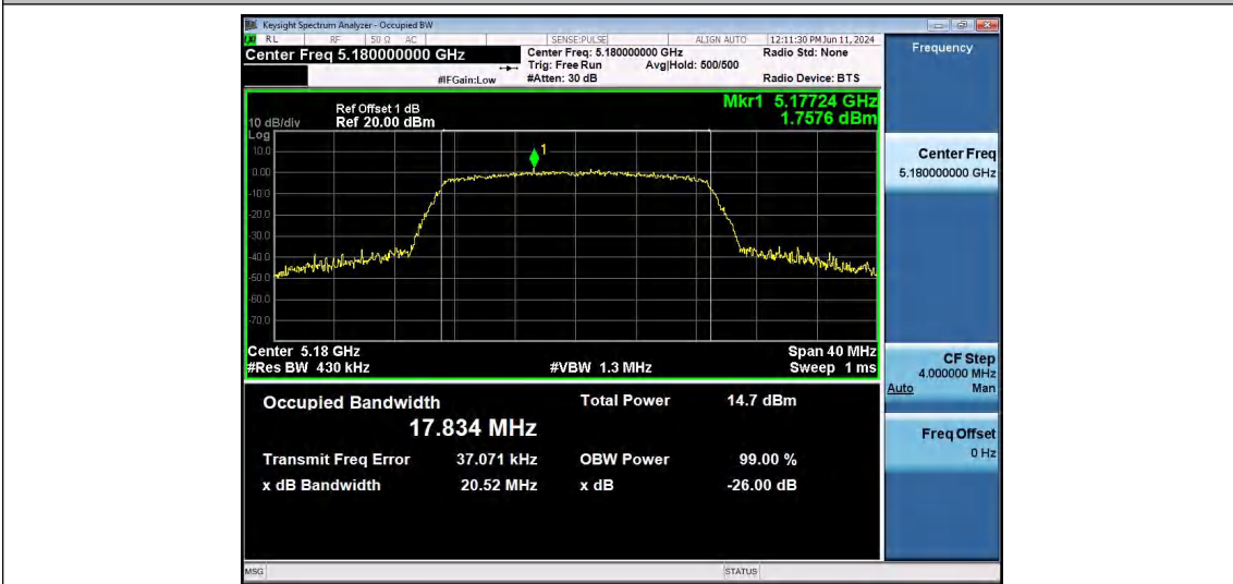
11AC20SISO-Ant1-5180
