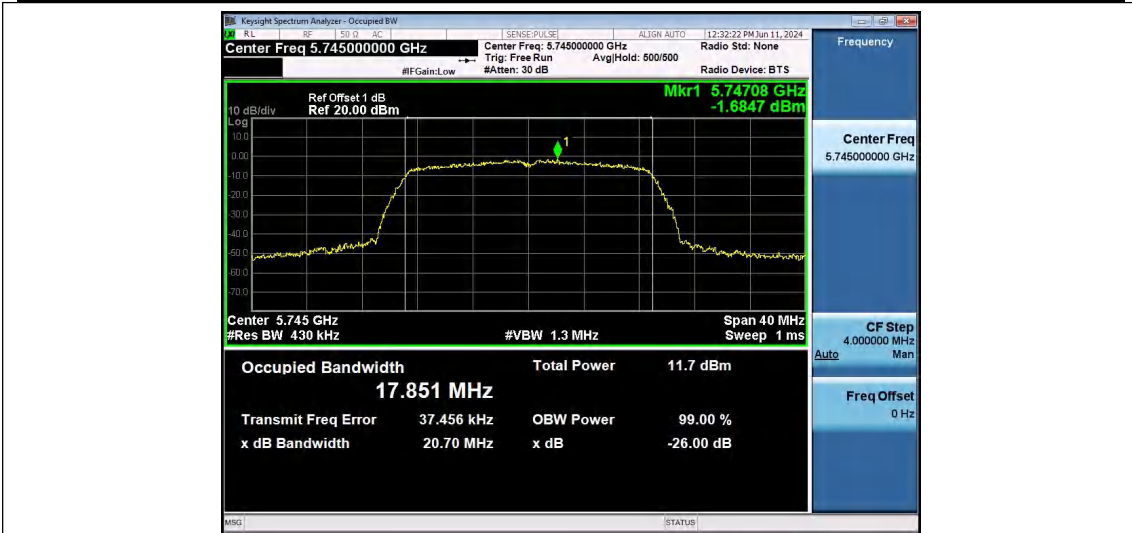
11N20SISO-Ant1-5745
