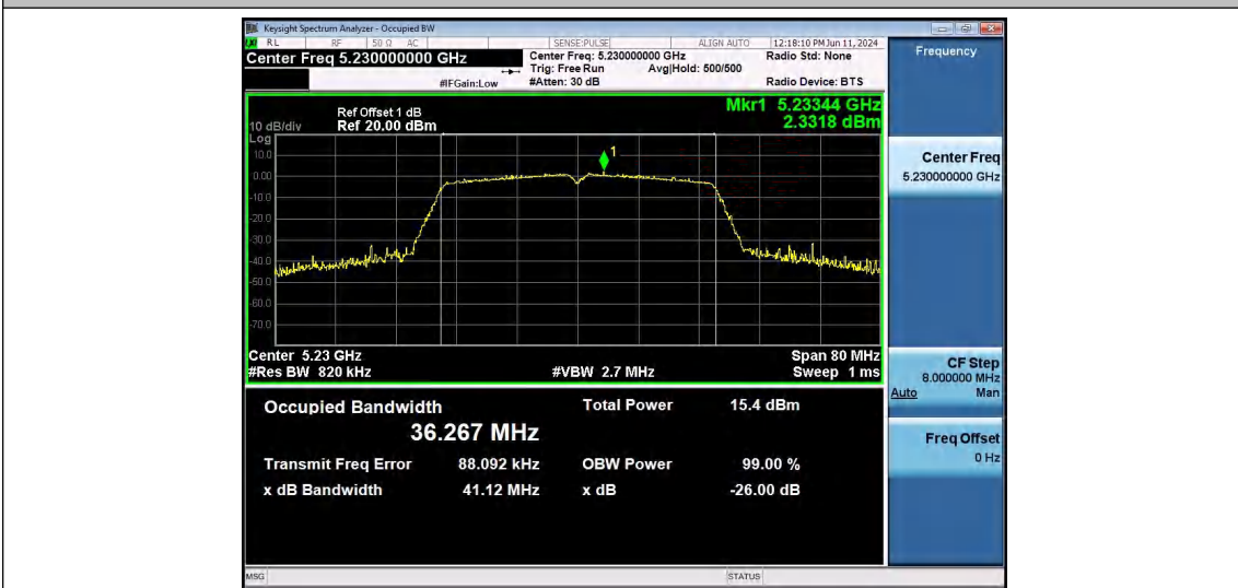
11AC40SISO-Ant1-5230
