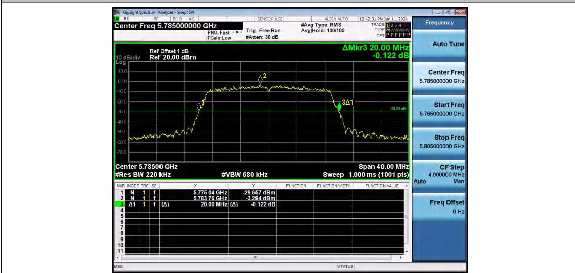
11AC20SISO-Ant1-5785
