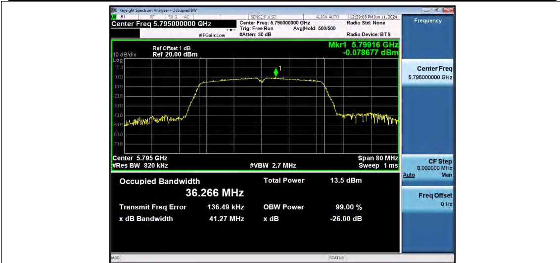
11N40SISO-Ant1-5795
