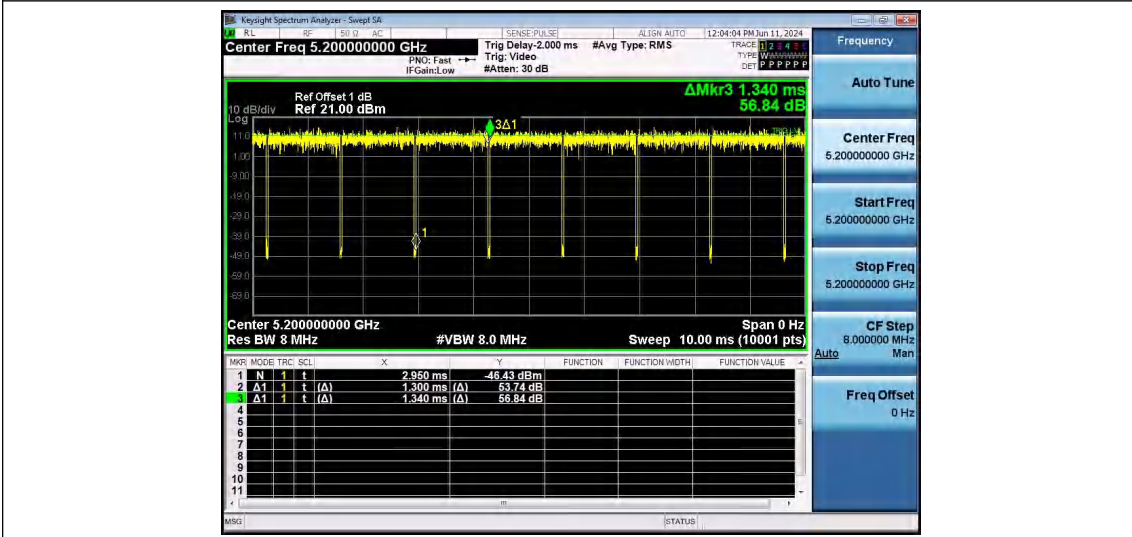
NTNV-11N20SISO-Ant1-5200
