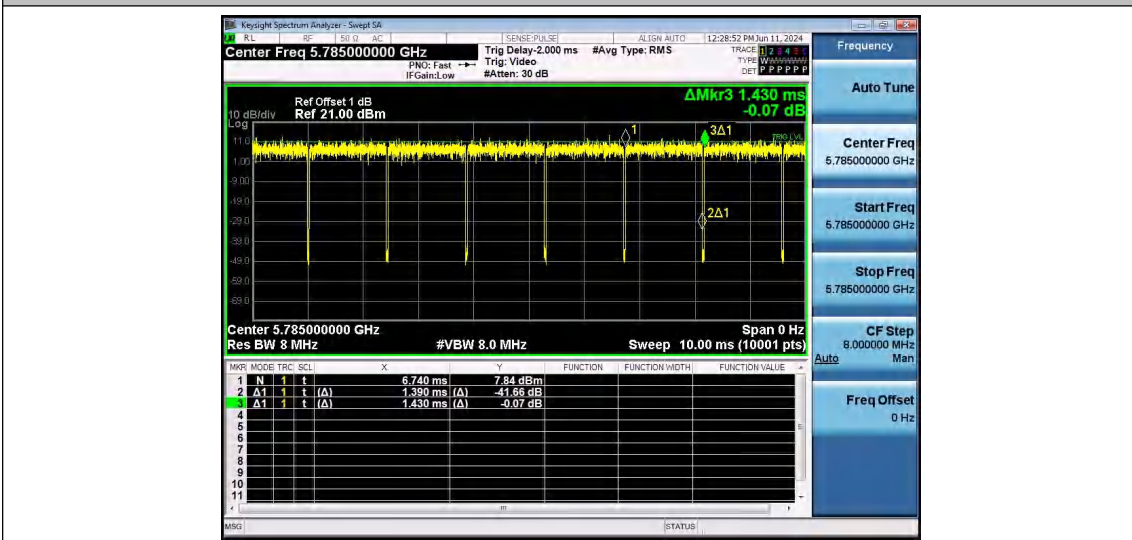
NTNV-11A-Ant1-5785
