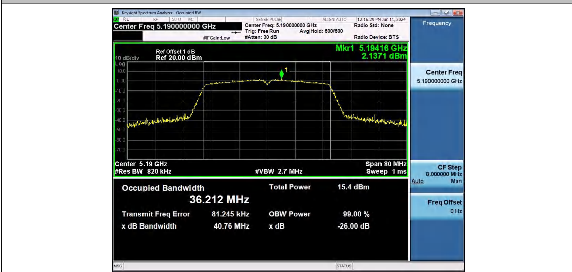
11AC40SISO-Ant1-5190
