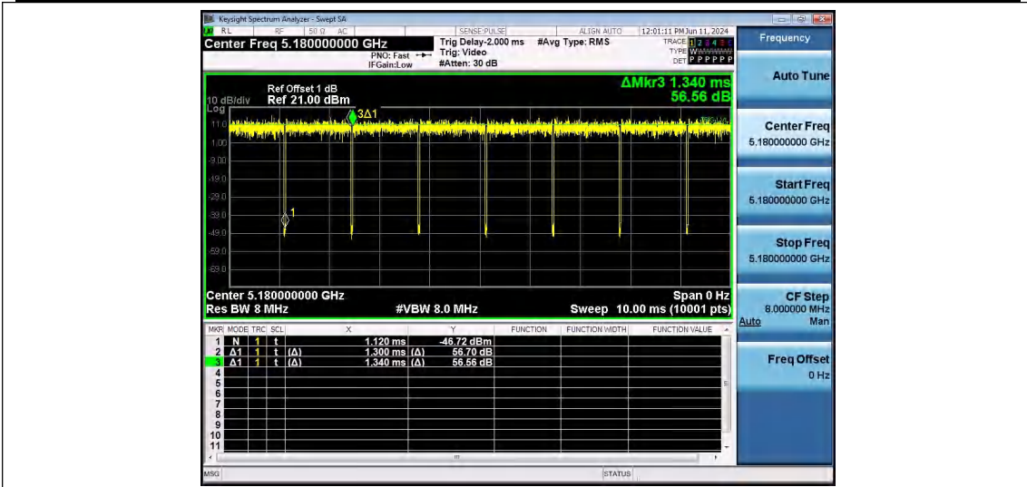
NTNV-11N20SISO-Ant1-5180
