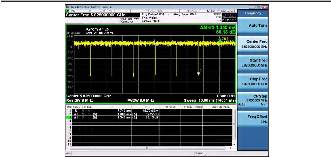
NTNV-11N20SISO-Ant1-5825
