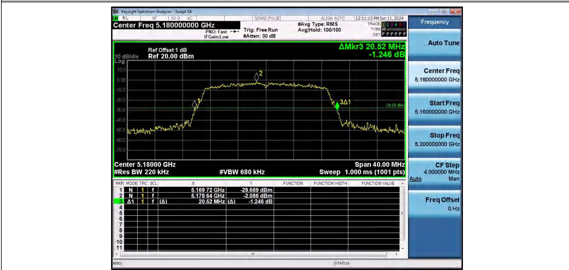
11AC20SISO-Ant1-5180
