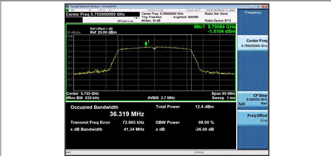
11N40SISO-Ant1-5755
