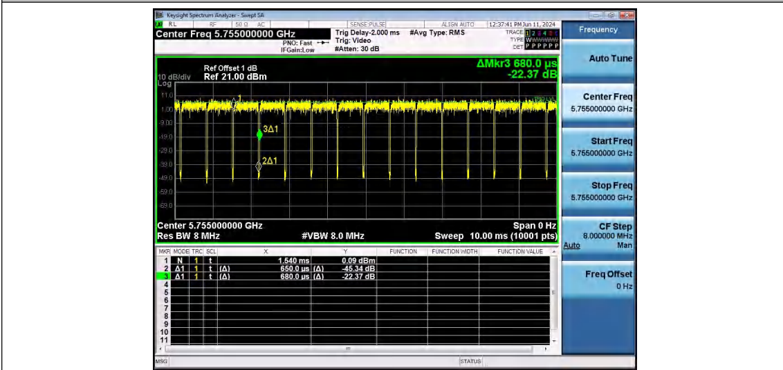
NTNV-11N40SISO-Ant1-5755
