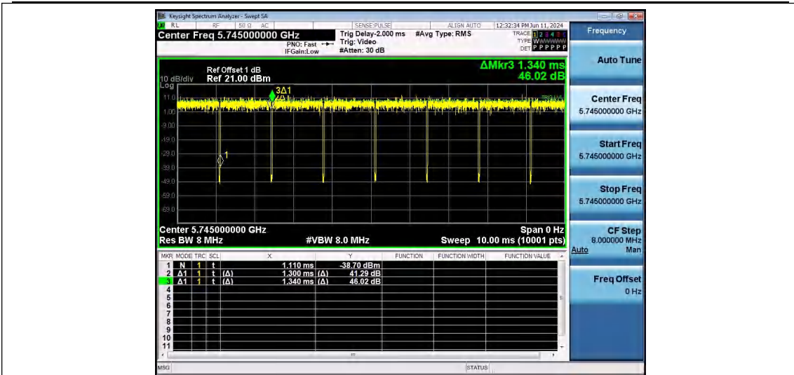
NTNV-11N20SISO-Ant1-5745
