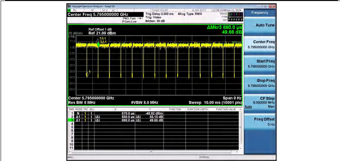
NTNV-11N40SISO-Ant1-5795
