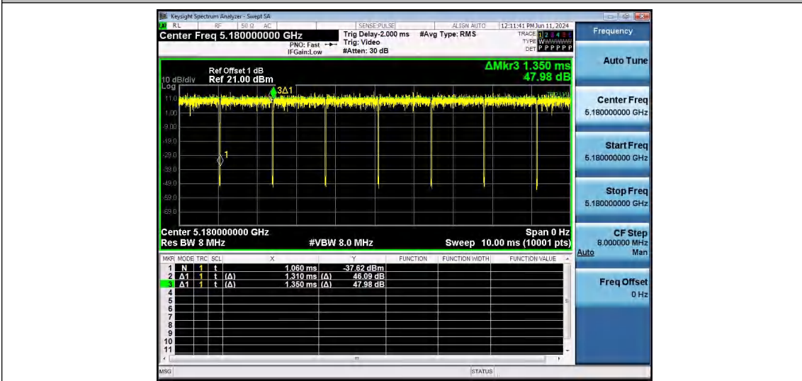
NTNV-11AC20SISO-Ant1-5180
