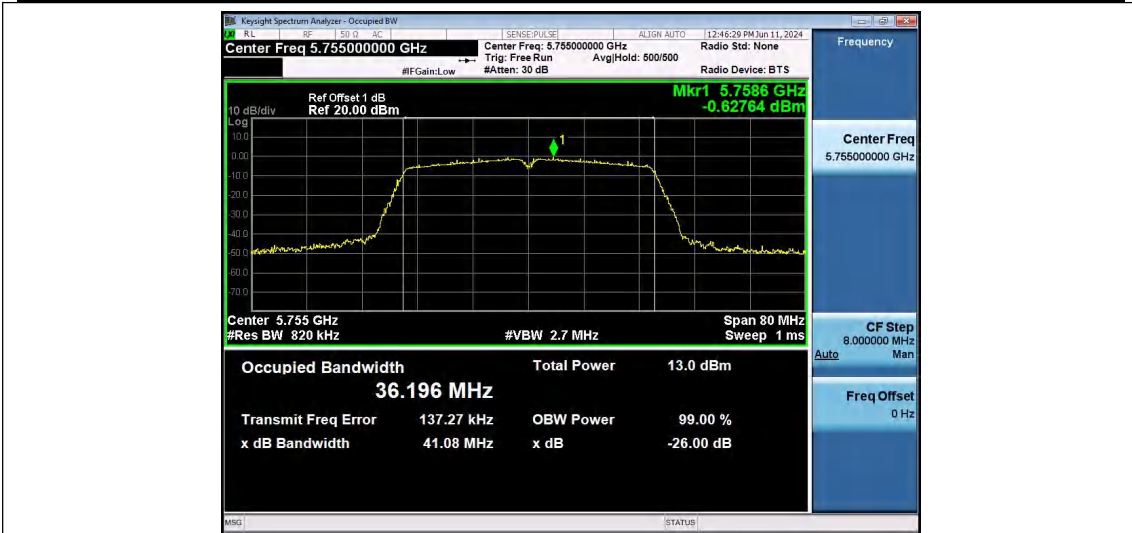
11AC40SISO-Ant1-5755
