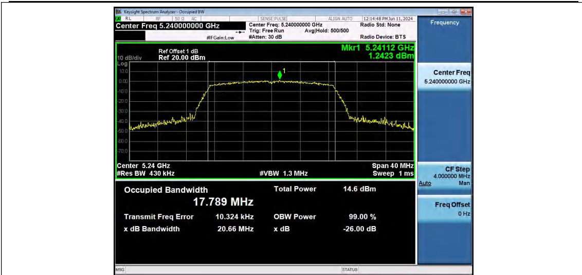
11AC20SISO-Ant1-5240
