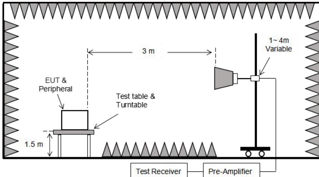
Figure 3. Above 1 GHz
