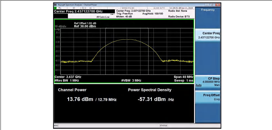
11B-Ant1-2437-PASS
