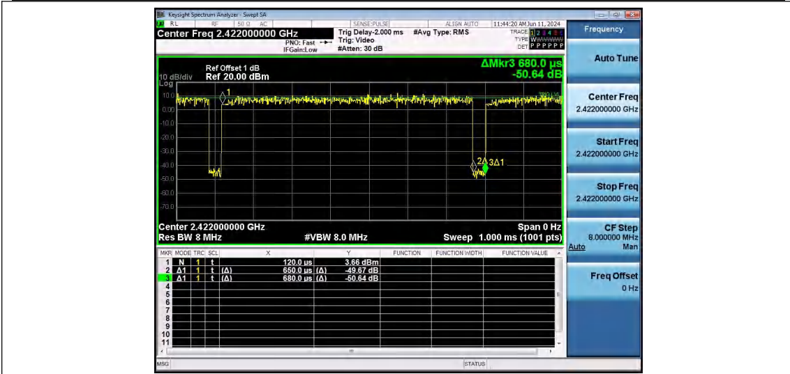
NTNV-11N40SISO-Ant1-2422
