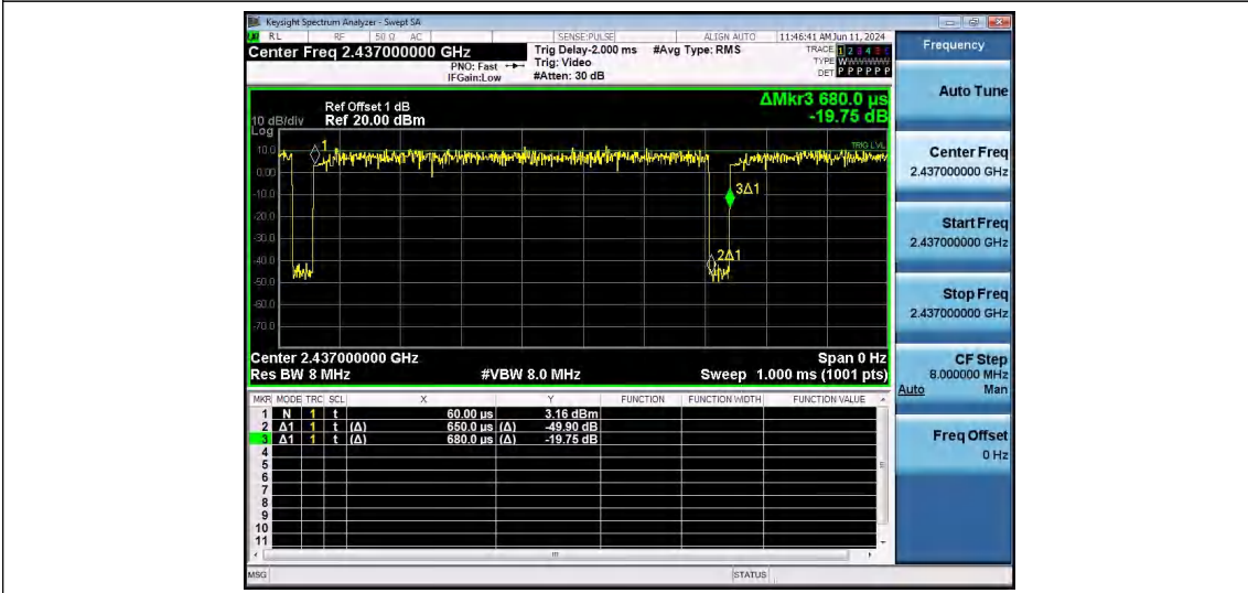
NTNV-11N40SISO-Ant1-2437
