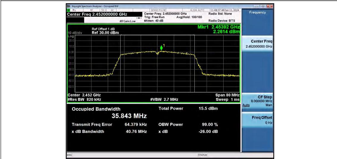
11N40SISO-Ant1-2452
