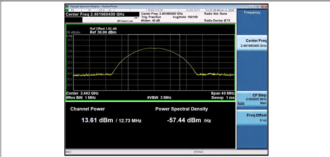
11B-Ant1-2462-PASS
