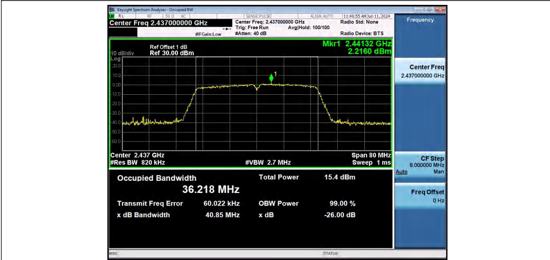
11N40SISO-Ant1-2437
