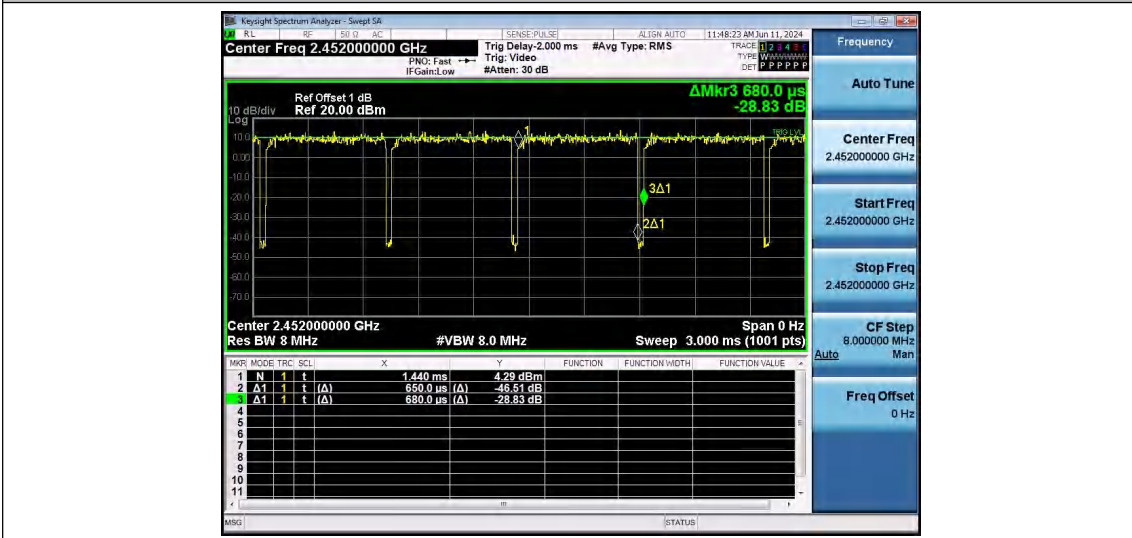
NTNV-11N40SISO-Ant1-2452
