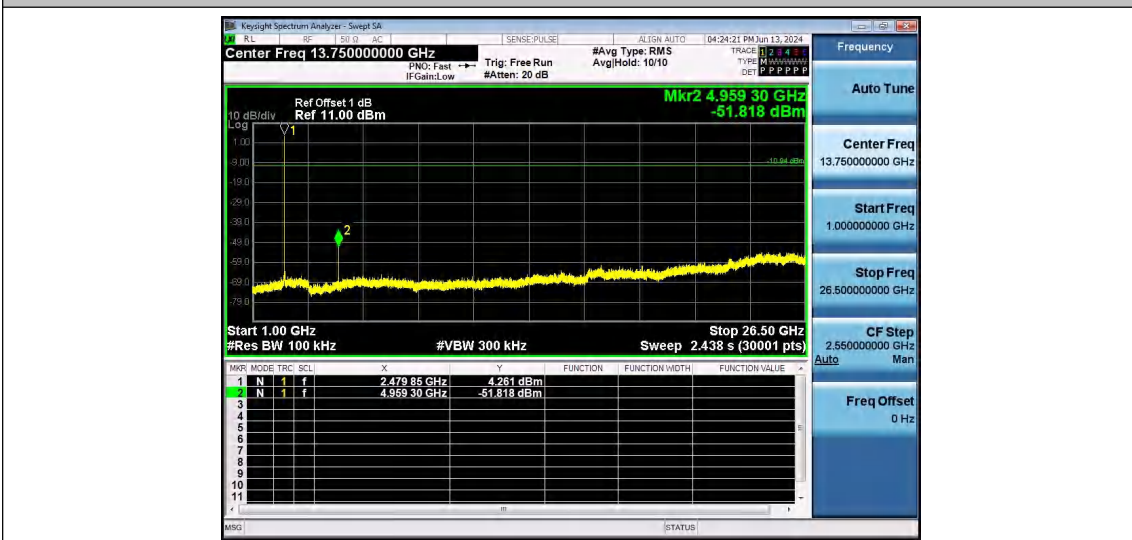
2DH5-Ant1-2480-1000~26500-PASS
