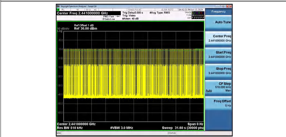
2DH1-Ant1-Hop-PASS
