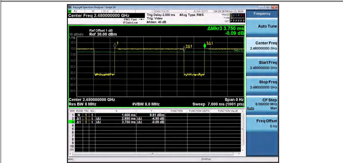
NTNV-3DH5-Ant1-2480
