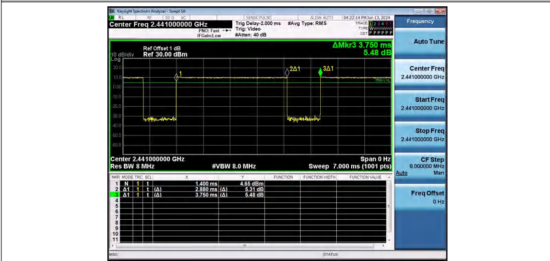
NTNV-2DH5-Ant1-2441
