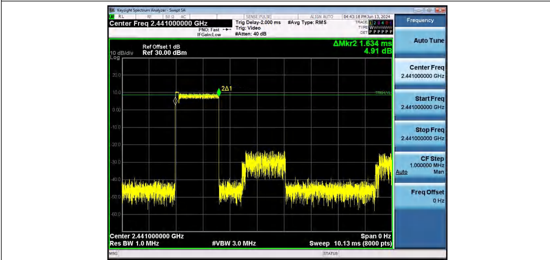
2DH3-Ant1-Hop-PASS
