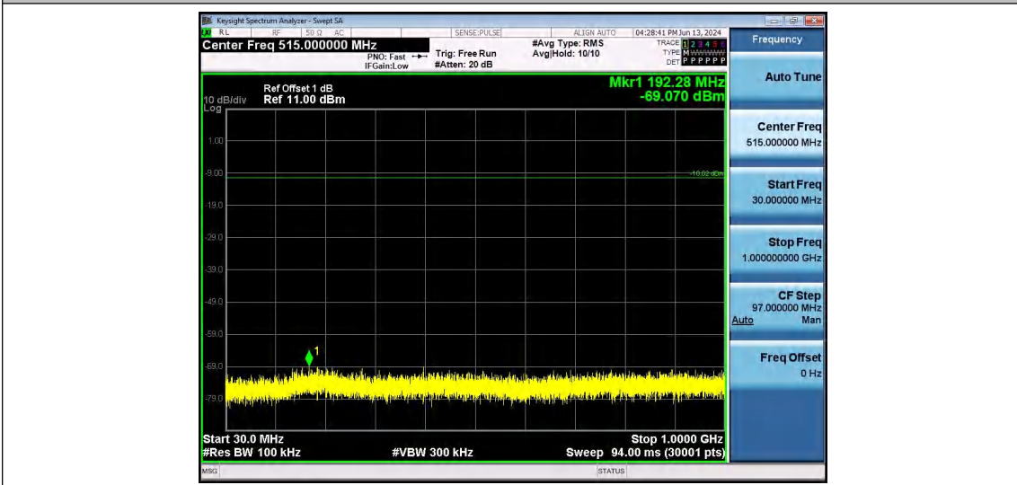
3DH5-Ant1-2441-30~1000-PASS
