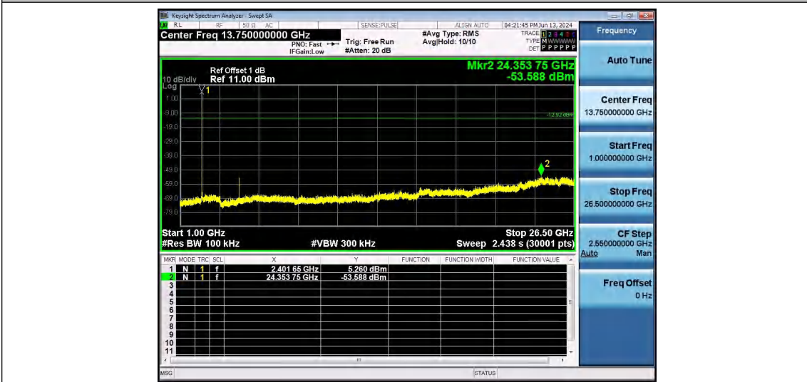
2DH5-Ant1-2402-1000~26500-PASS
