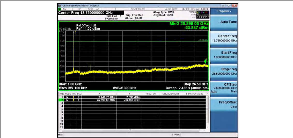
3DH5-Ant1-2441-1000~26500-PASS
