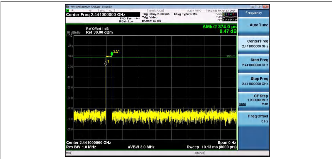
DH1-Ant1-Hop-PASS
