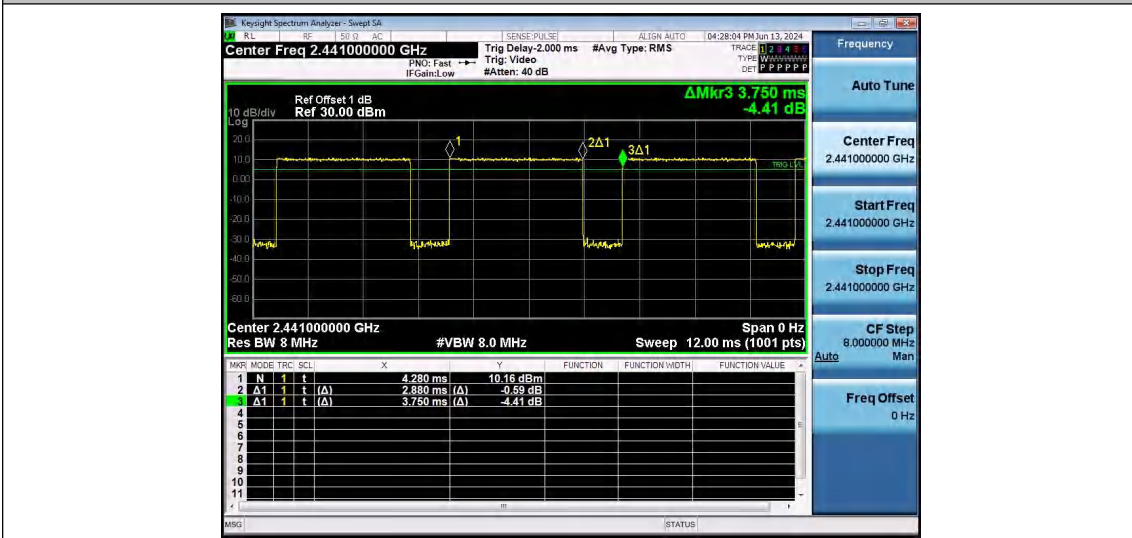
NTNV-3DH5-Ant1-2441
