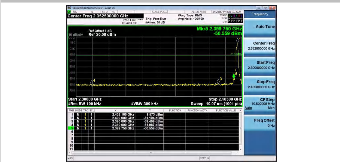
3DH5-Ant1-2402-PASS
