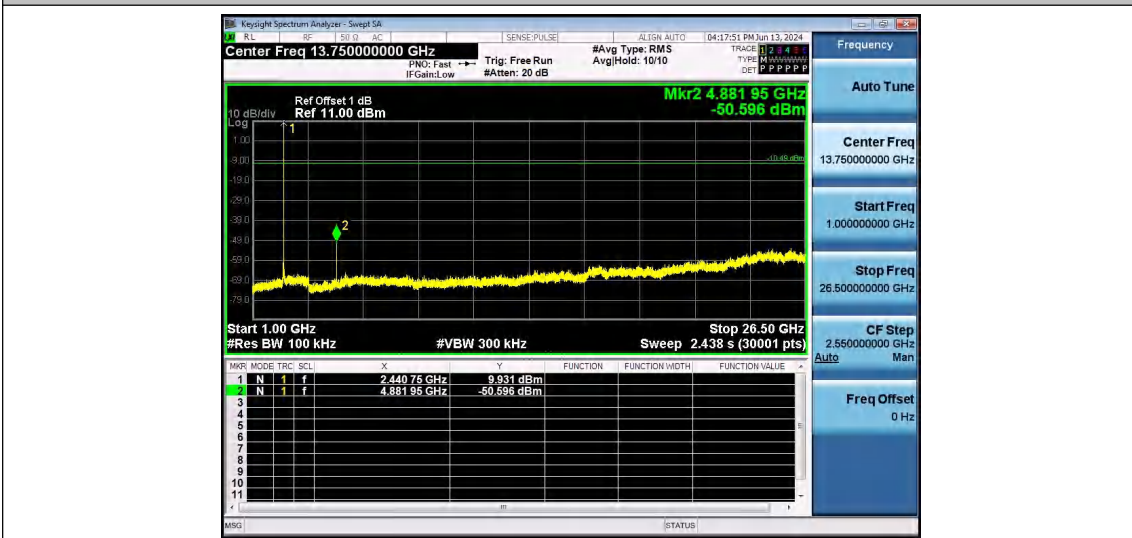
DH5-Ant1-2441-1000~26500-PASS
