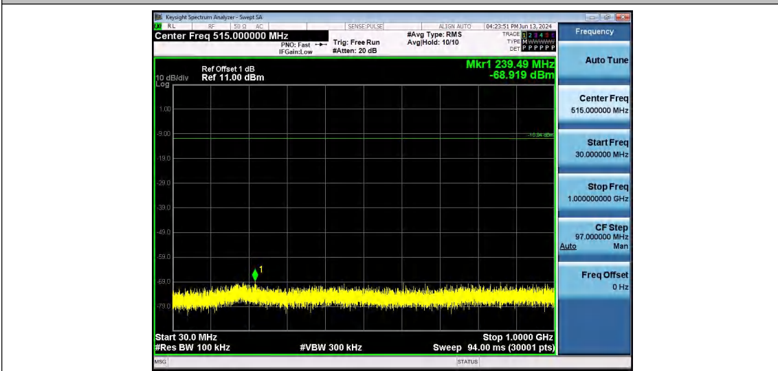
2DH5-Ant1-2480-30~1000-PASS
