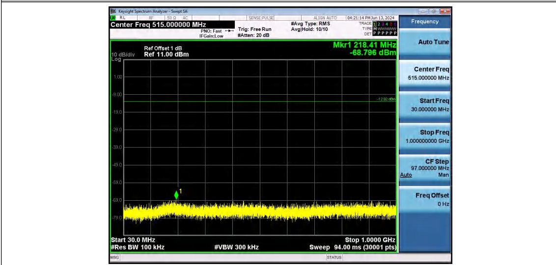
2DH5-Ant1-2402-30~1000-PASS
