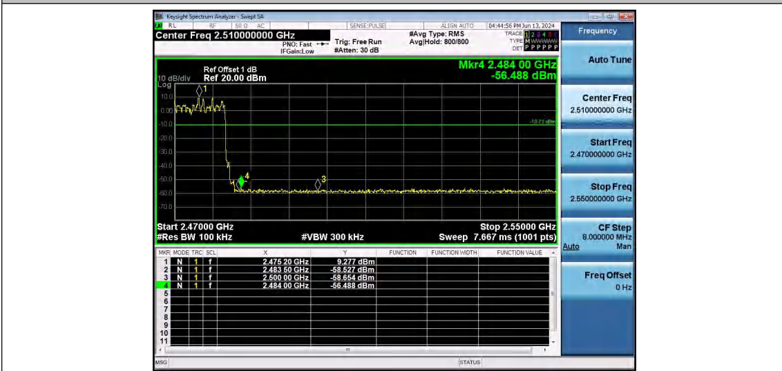
3DH5-Ant1-Hop_2480-PASS
