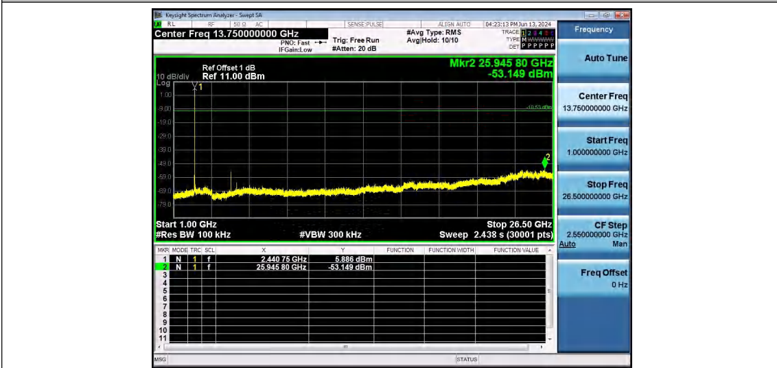
2DH5-Ant1-2441-1000~26500-PASS
