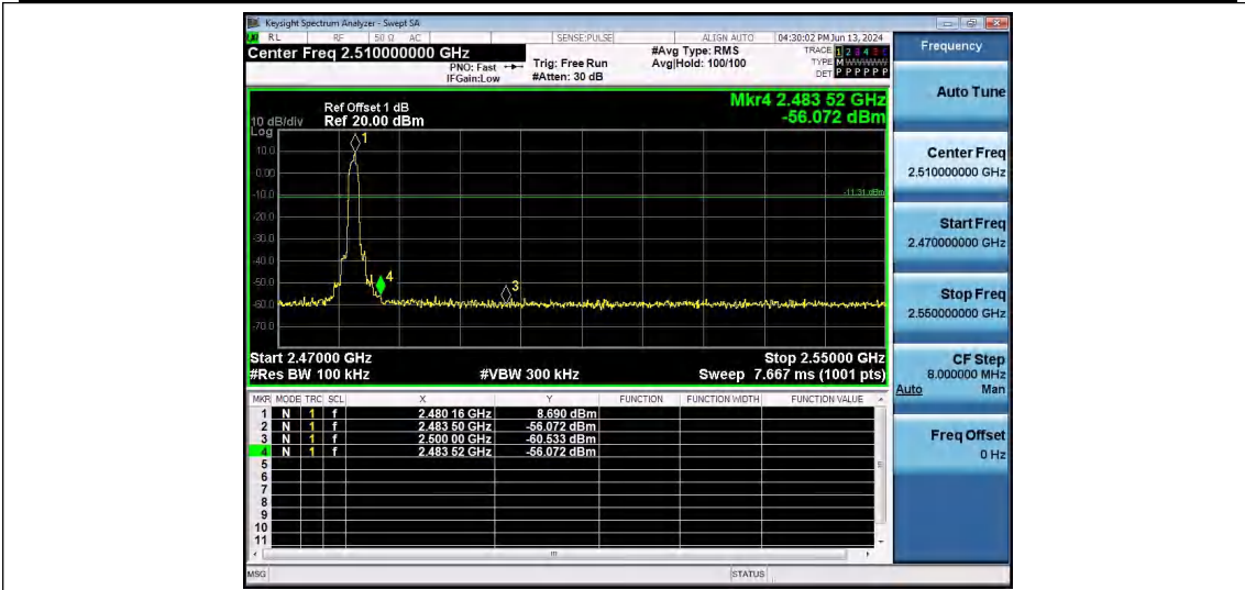
3DH5-Ant1-2480-PASS
