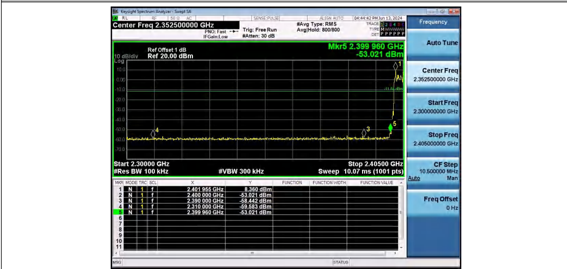
3DH5-Ant1-Hop_2402-PASS
