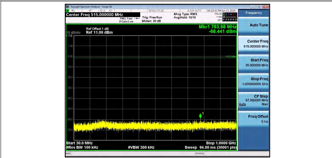
2DH5-Ant1-2441-30~1000-PASS
