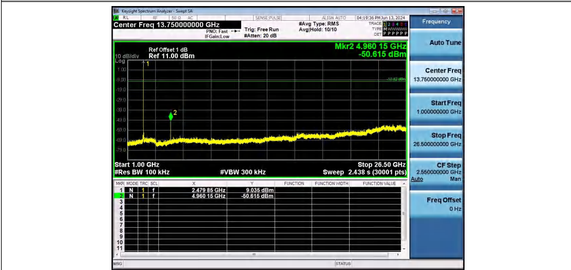
DH5-Ant1-2480-1000~26500-PASS
