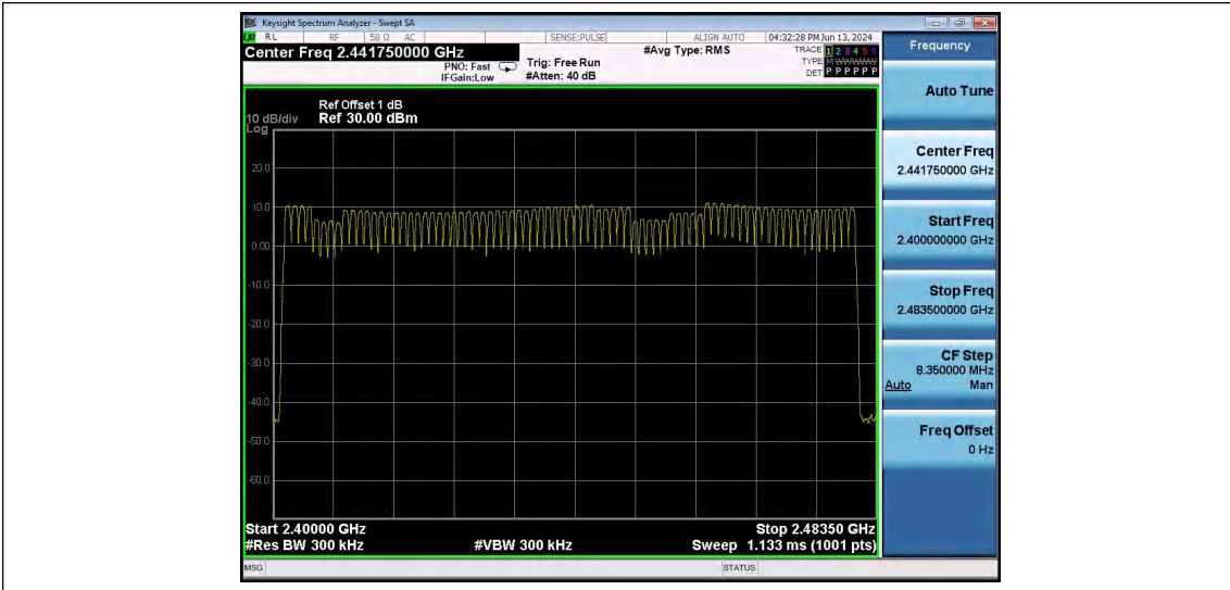
DH5-Ant1-Hop-PASS
