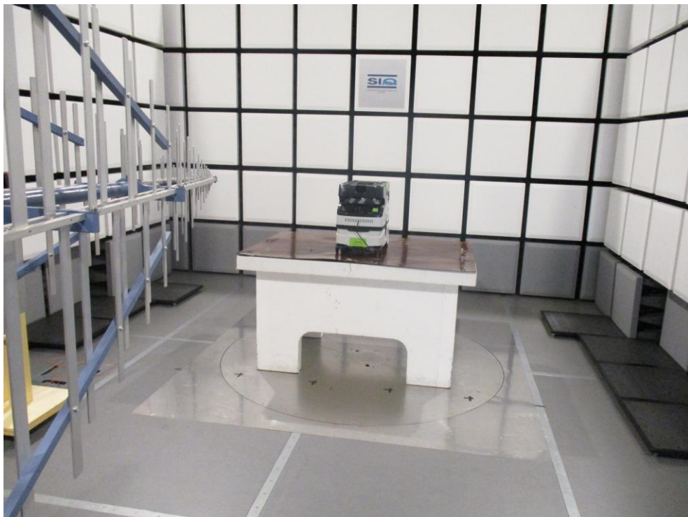
Figure 2: Spurious emission 30 MHz-1000 MHz
