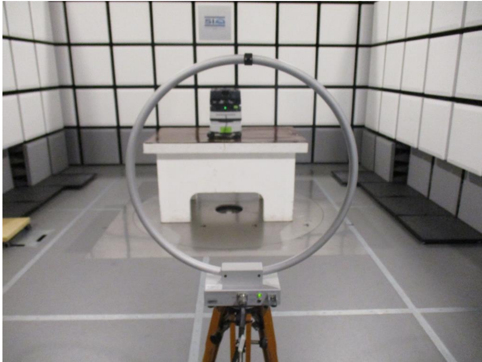
Figure 1: Spurious emission 9 kHz-30 MHz
