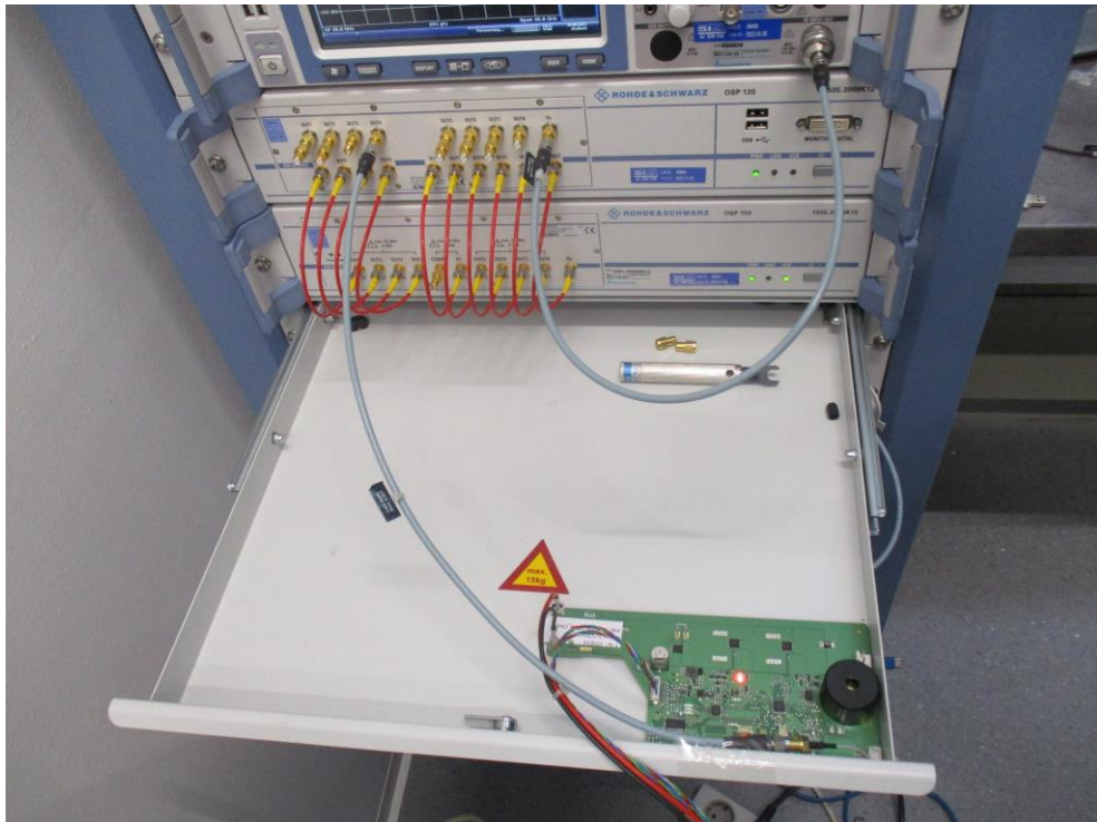
Figure 5: Conducted measurements test setup
