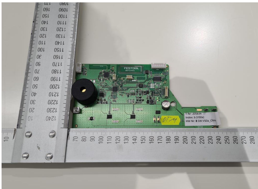
Figure 2: Sample for radiated measurements
