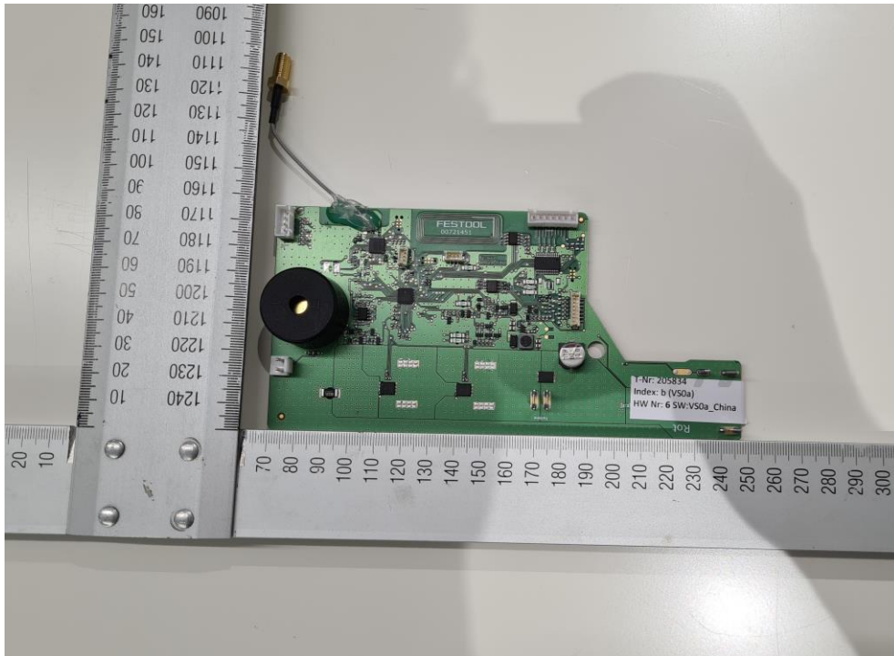
Figure 3: Modified sample for conducted measurements
