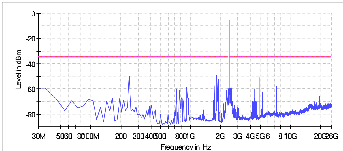
Sourious
