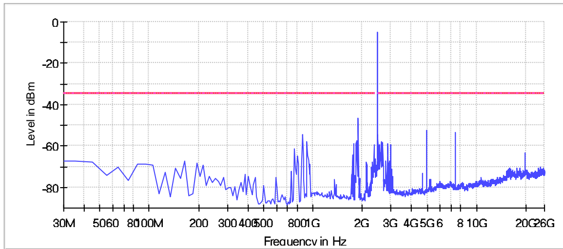
Sourious
