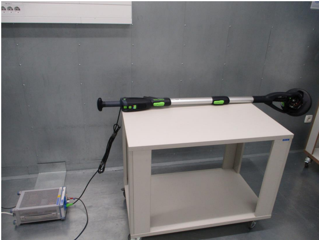
Figure 1:Conducted emission
