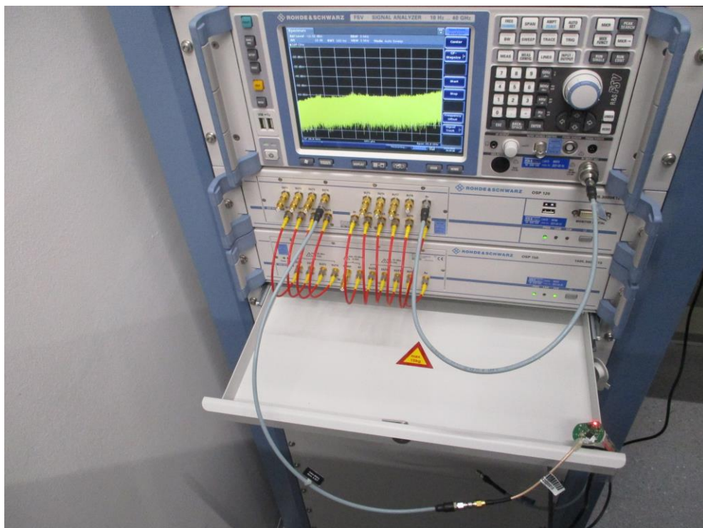
Figure 6: Conducted measurements test setup
