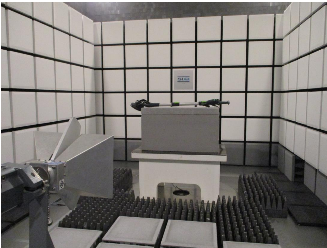
Figure 4: Spurious emission 1-18 GHz
