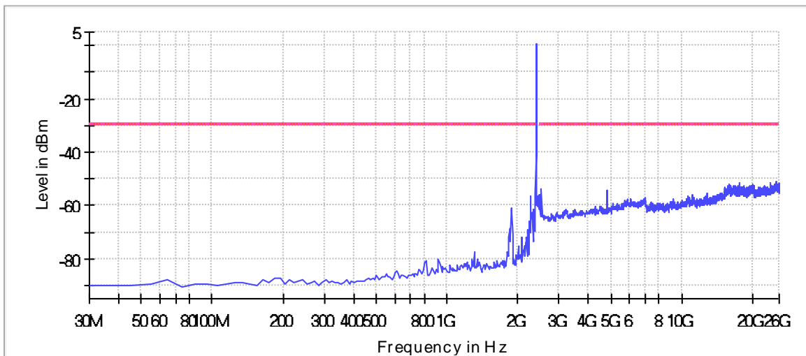
Spurious
