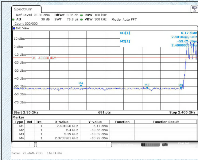
2DH5(2402)-Hopping on
