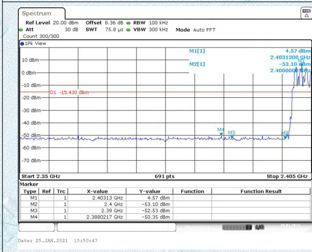
3DH5(2402)-Hopping on
