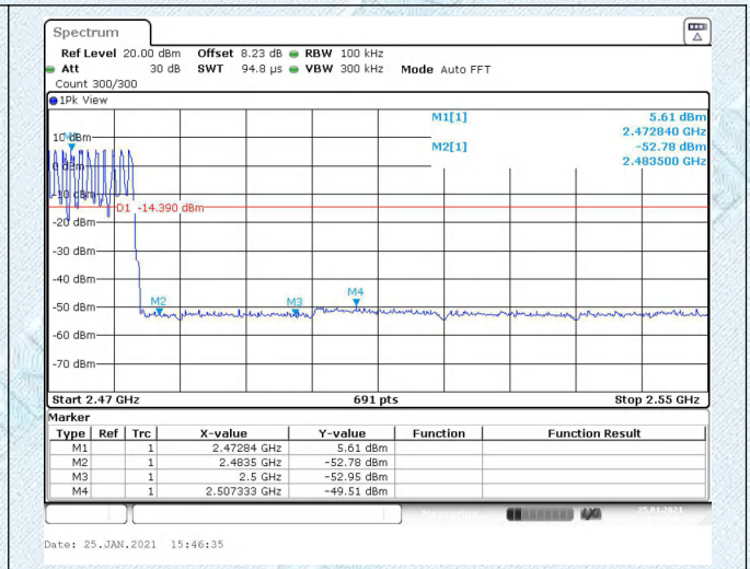
2DH5(2480)-Hopping on
