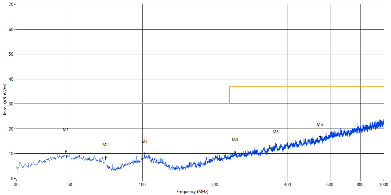
RE Test Case_CE Certification_EN 55032 Class B 30MHz-1GHz
