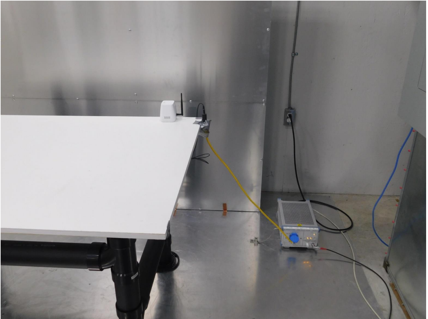
Conducted 150 kHz - 30 MHz ALF-000045 (sensor)
