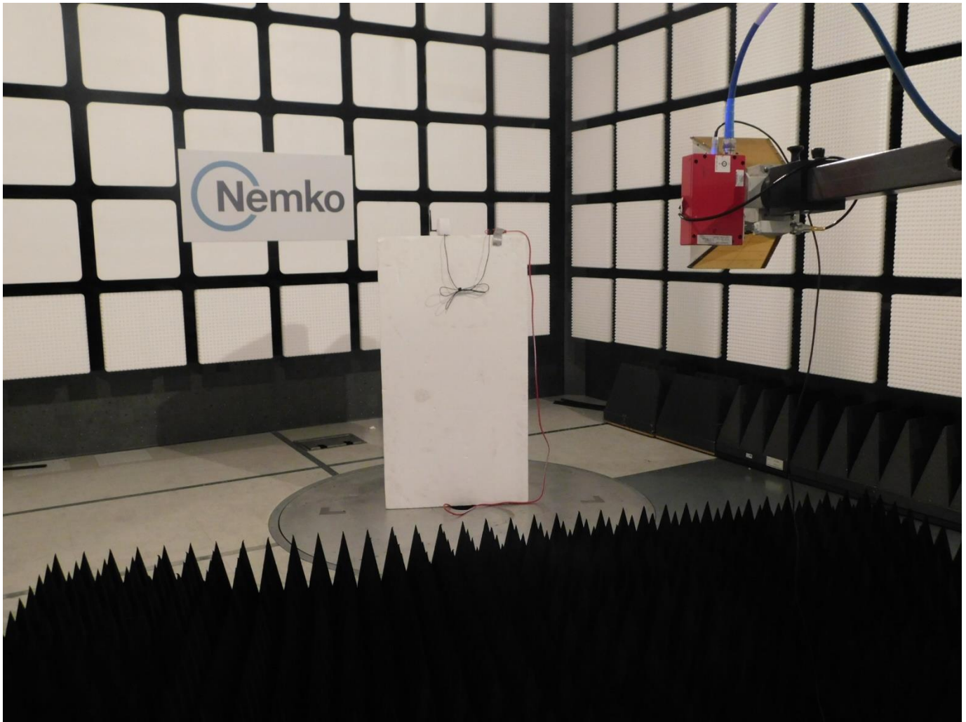
Radiated 1-10 GHz ALF-000045 (sensor)
