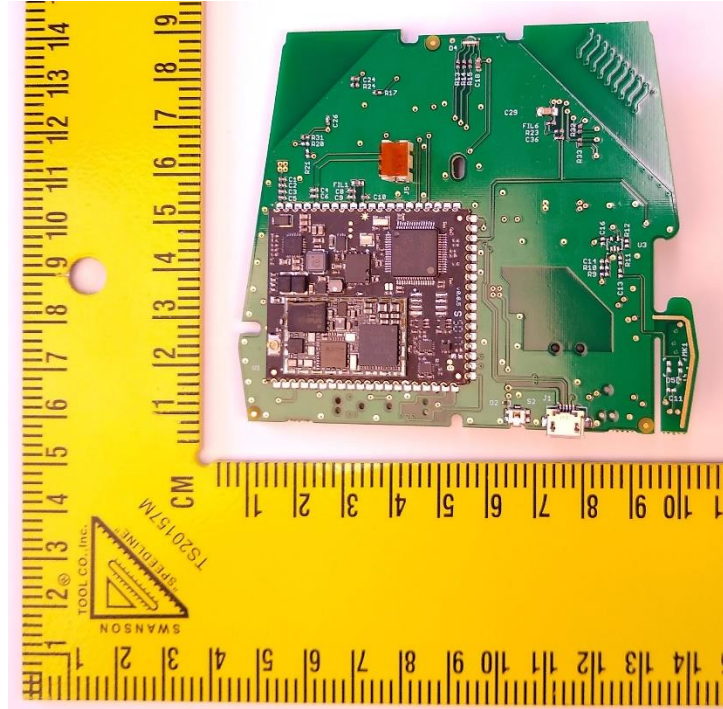
Figure 7: Sensor Relay (ALF-000045 / ALF-000046) BOTTOM Layer, No Cans
