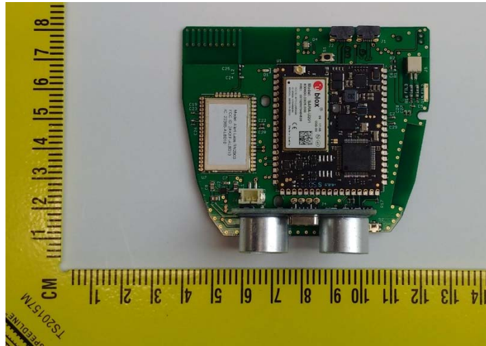
Figure 1: Top Side
