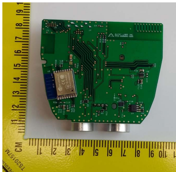
Figure 2: Bottom Side
