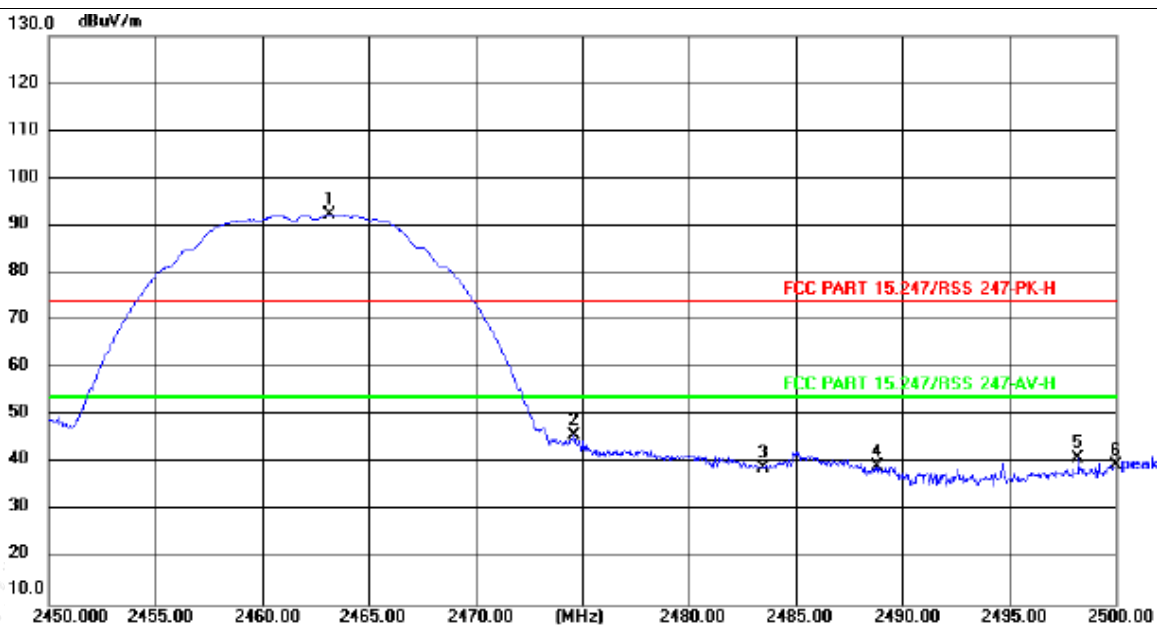
Restrict Band NVNT b 2462MHz Ant Peak- Horizontal
