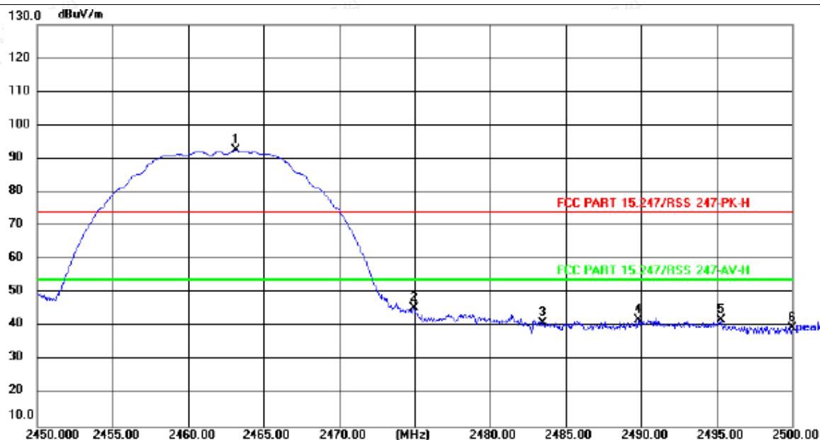
Restrict Band NVNT b 2462MHz Ant Peak- Vertical
