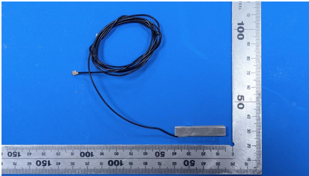
Antenna 2 (Chain 1)
