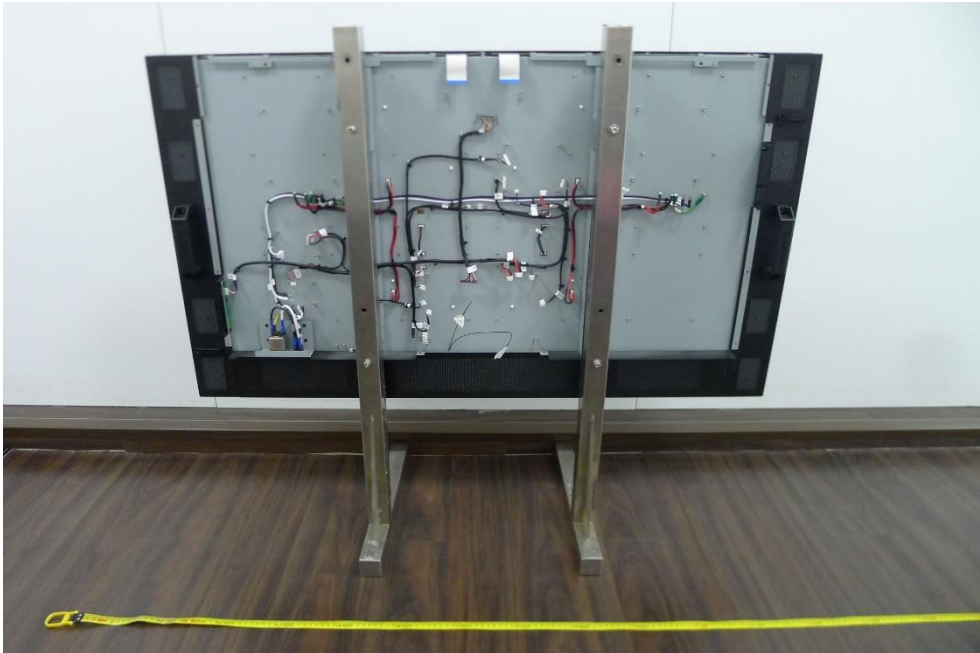
(26) EUT Photo
