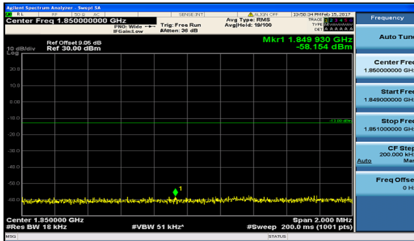
(Channel Bandwidth:20 MHz)_LCH_QPSK_1RB#99
