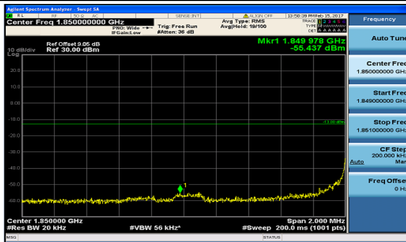
(Channel Bandwidth:20 MHz)_LCH_QPSK_50RB#0
