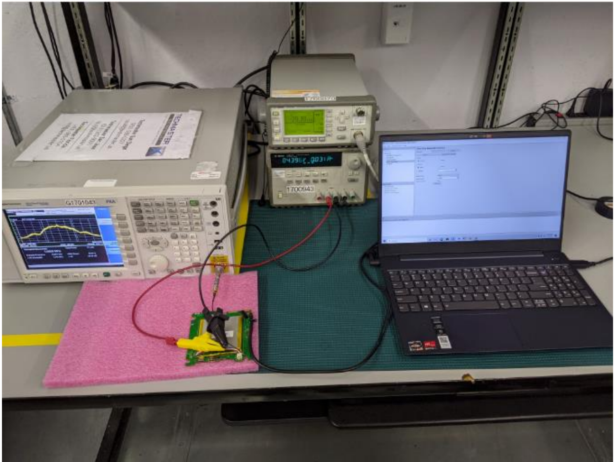
Figure 3: RF Conducted Test Setup
