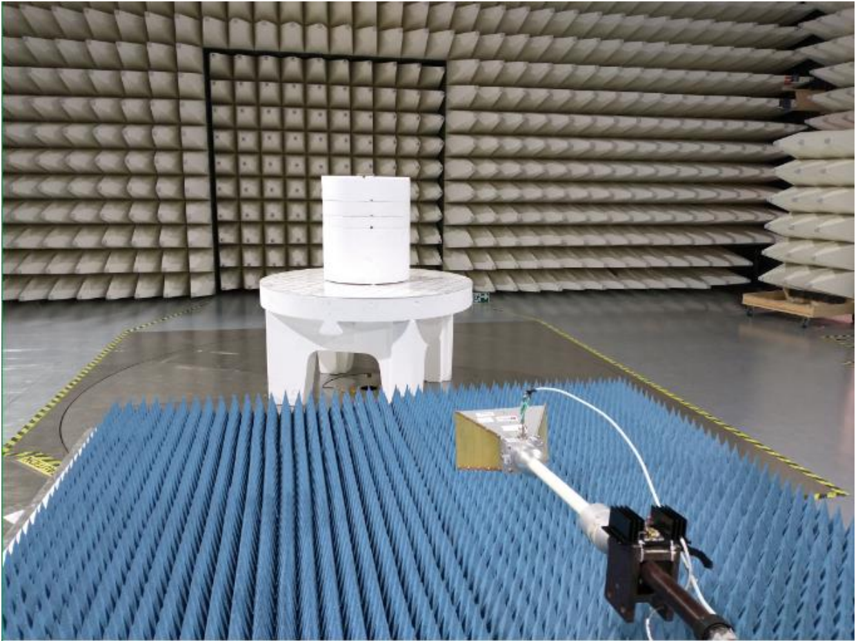
Figure 2: Test Setup for 1GHz to 18GHz (Rear View)
