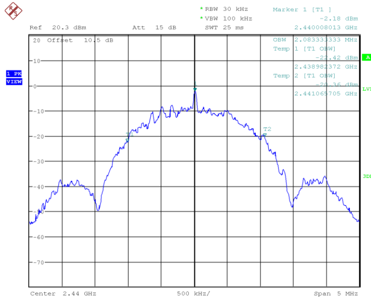
Figure 17: 2440MHz, 2Mbps, 99% Bandwidth
