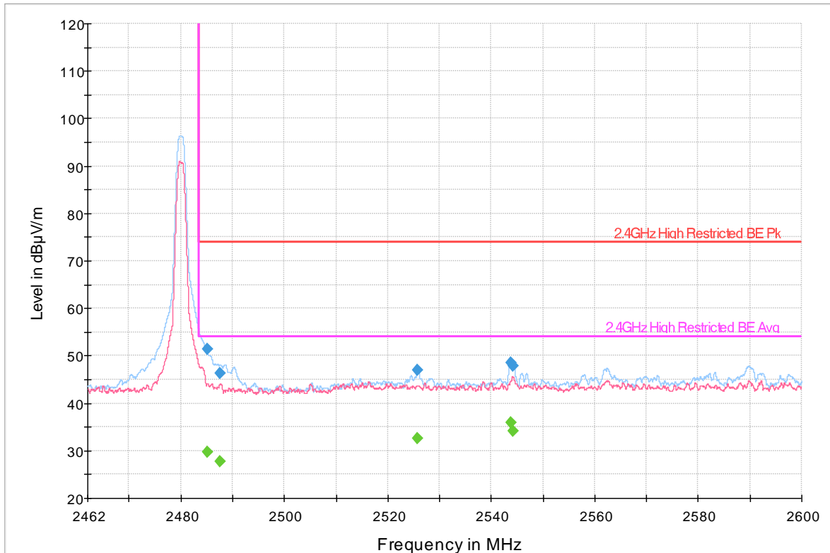
— Preview Result 1H-PK+ — Preview Result 1V-PK+ — 2.4GHz High Restricted BE Pk — 2.4GHz High Restricted BE Ava ◆ Final_Result PK+ ◆ Final_Result AVG
