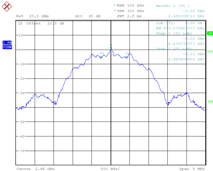
Figure 12: 2480MHz, 2Mbps, 6dB Bandwidth
