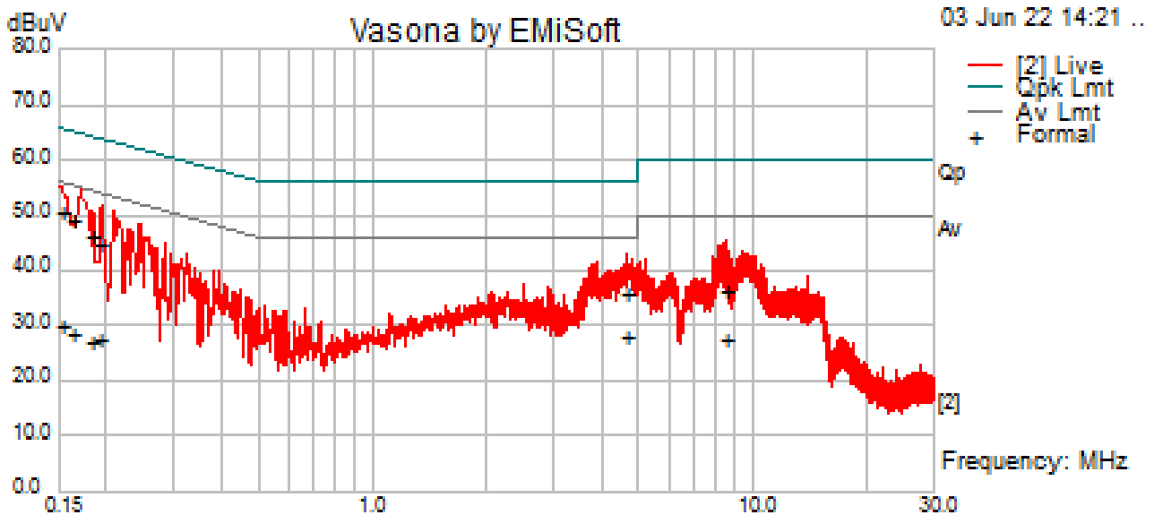
Figure 48: AC Conducted Emissions 150 kHz to 30 MHz-Live Line
