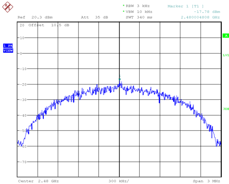
Figure 24: 2480MHz, 2Mbps, PSD
