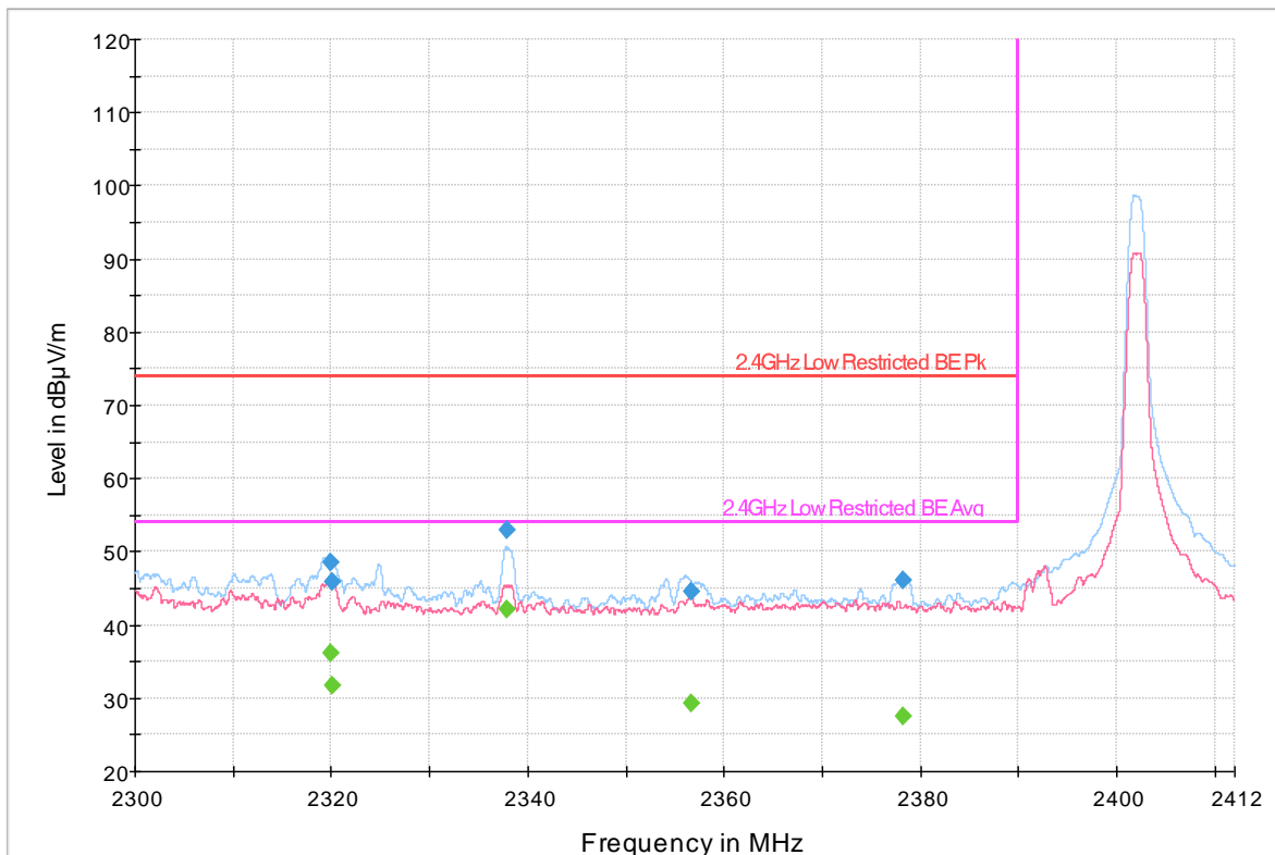
— Preview Result 1H-PK+ — Preview Result 1V-PK+ — 2.4GHz Low Restricted BE PK — 2.4GHz Low Restricted BE Avg ◆ Final_Result PK+ ◆ Final_Result AVG
