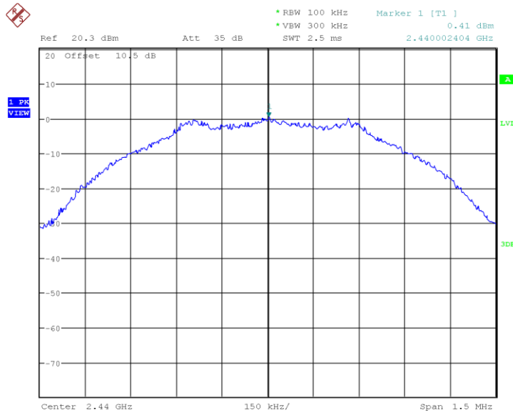
Figure 29: 1Mbps Ref Measurement
