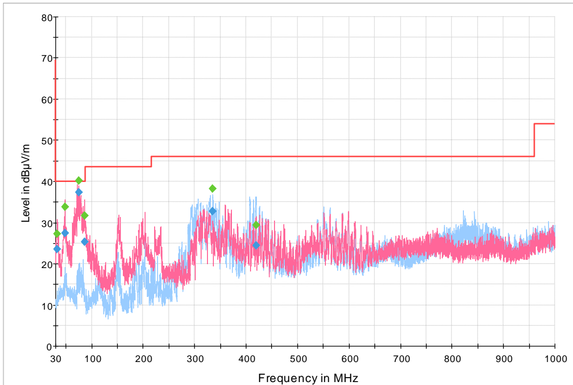
◆ Preview Result 1H-PK+ Final_Result QPK ◆ Preview Result 1V-PK+ Final_Result PK+ — FCC 15_QP
