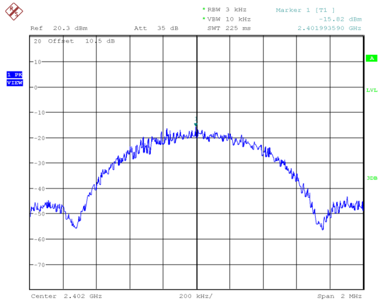
Figure 19: 2402 MHz, 1Mbps, PSD
