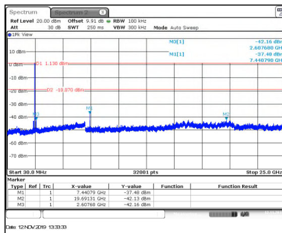
Figure 7.5.1.2-3: HCH – 30MHz–25GHz
