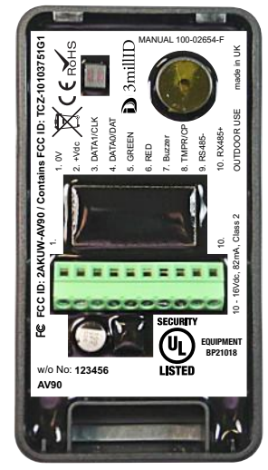
VIEW - REVERSE ▲ internal view assembled and POTTED
