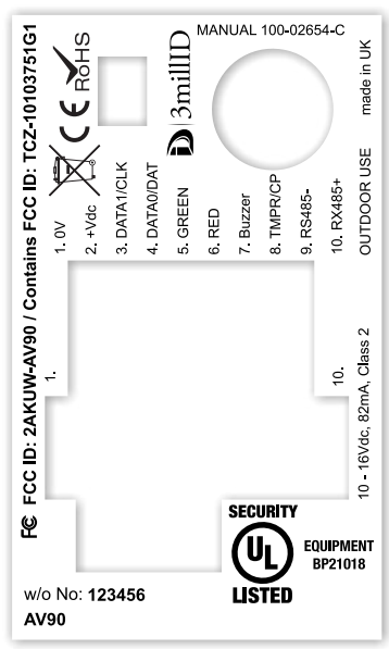
VIEW - REVERSE ▲ standard label format and layout
