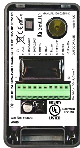
VIEW - REVERSE ▲ internal view assembled and POTTED
