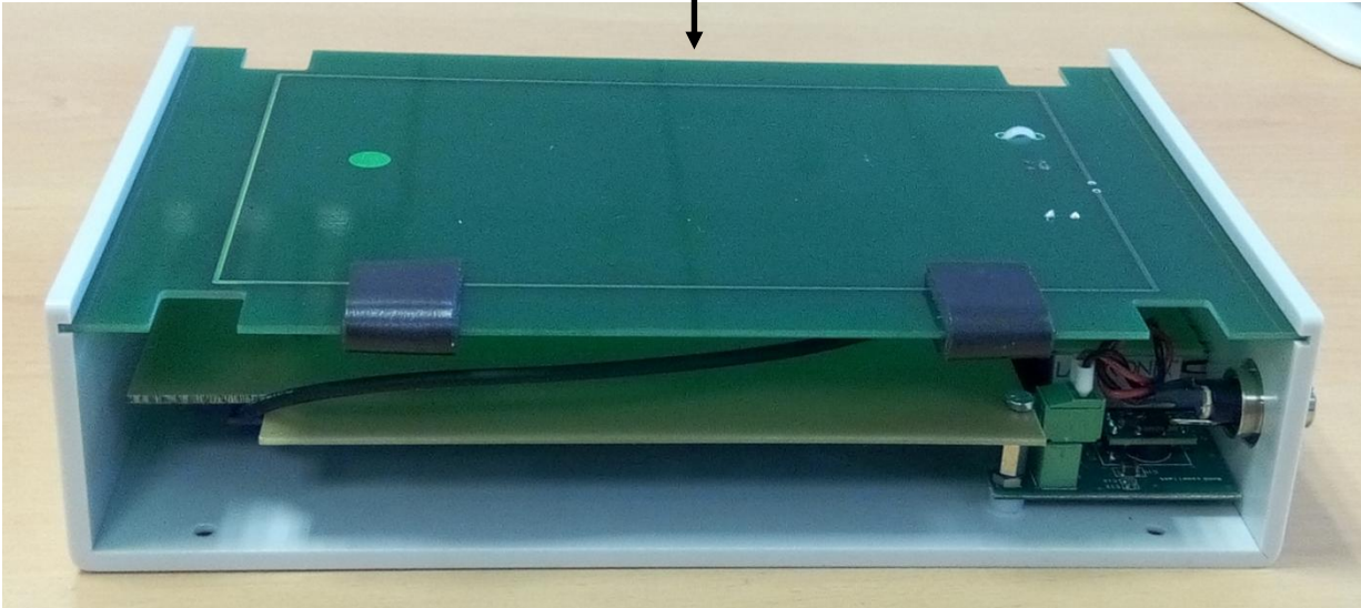
CAR_73103C: HF ANTENNA BOARD 211,5mm x 136mm
