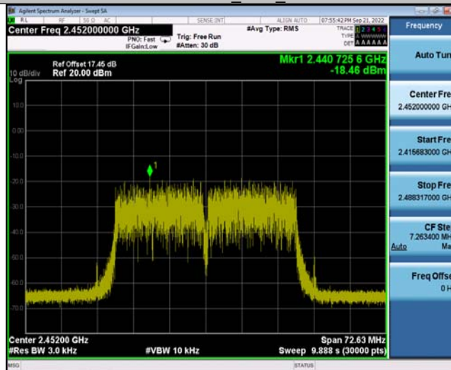
11N40SISO_Ant1_2452
