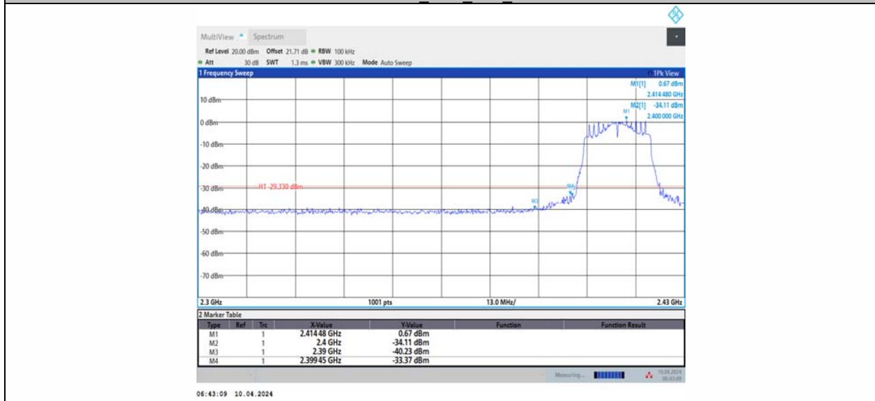
11N20SISO Ant1_Low_2412
