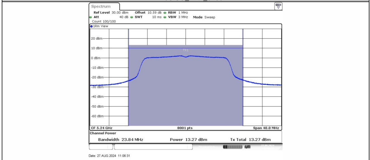
11N20SISO_Ant1_5240
