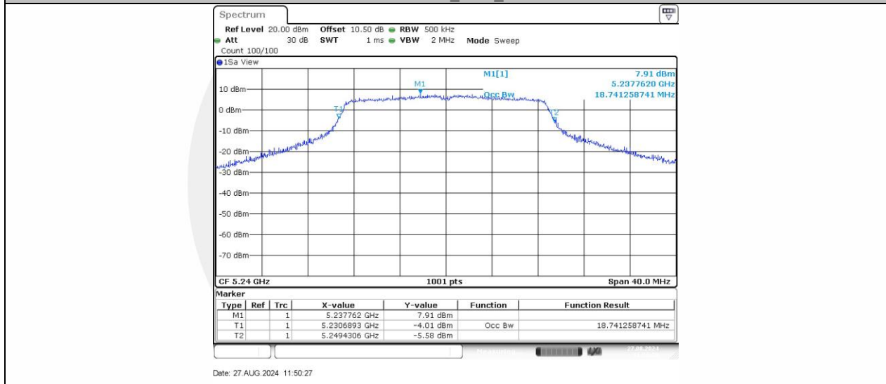
11AC20SISO_Ant1_5240
