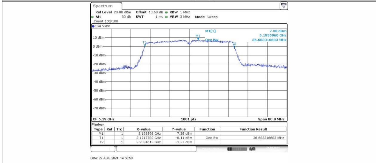
11AC40SISO_Ant1_5190
