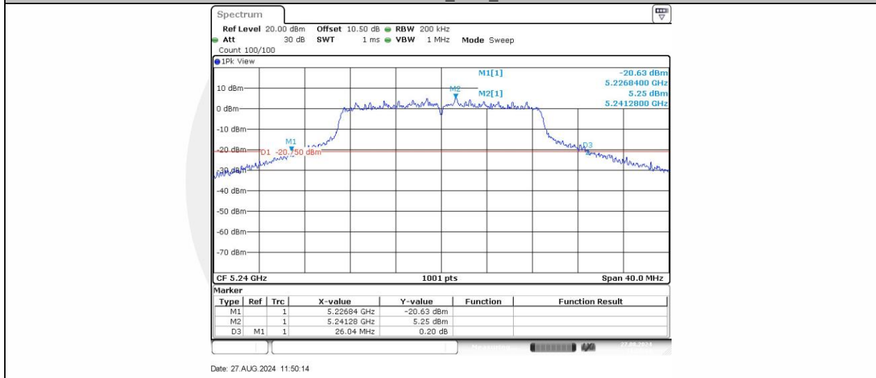
11AC20SISO_Ant1_5240
