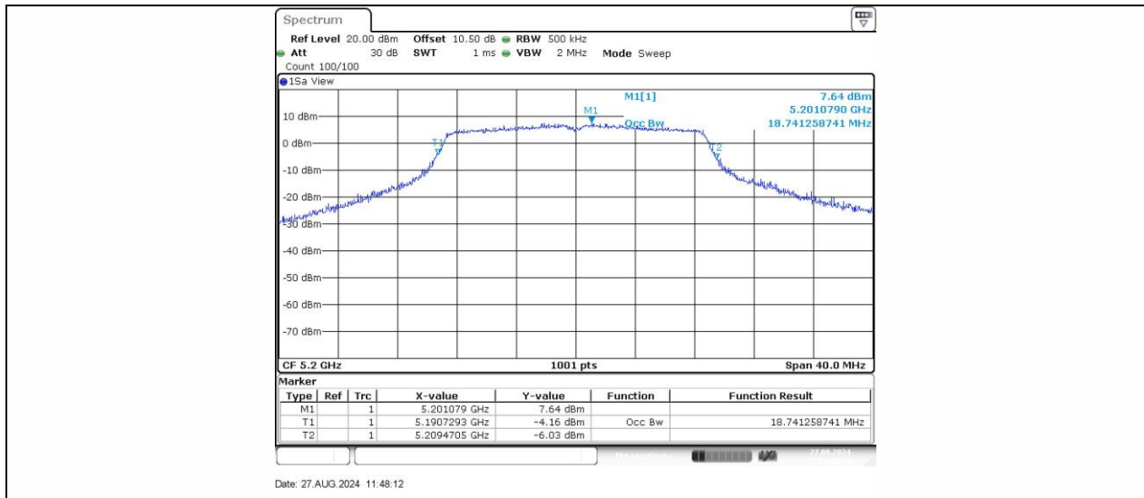
11AC20SISO_Ant1_5200
