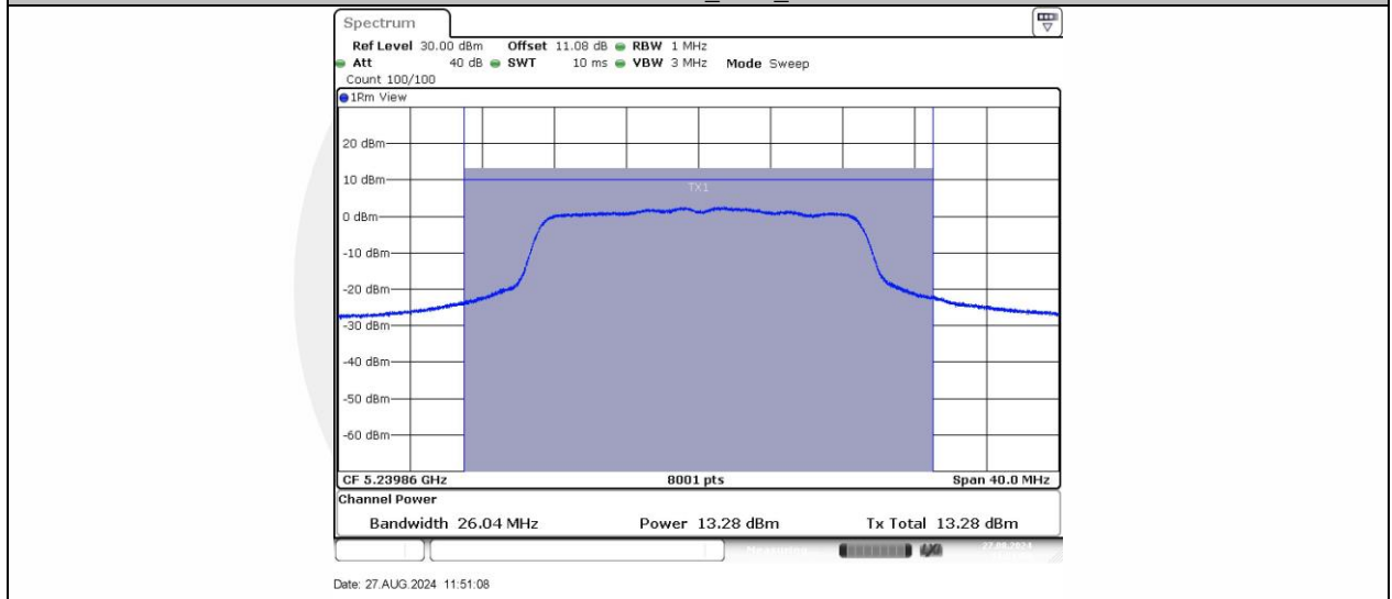
11AC20SISO_Ant1_5240
