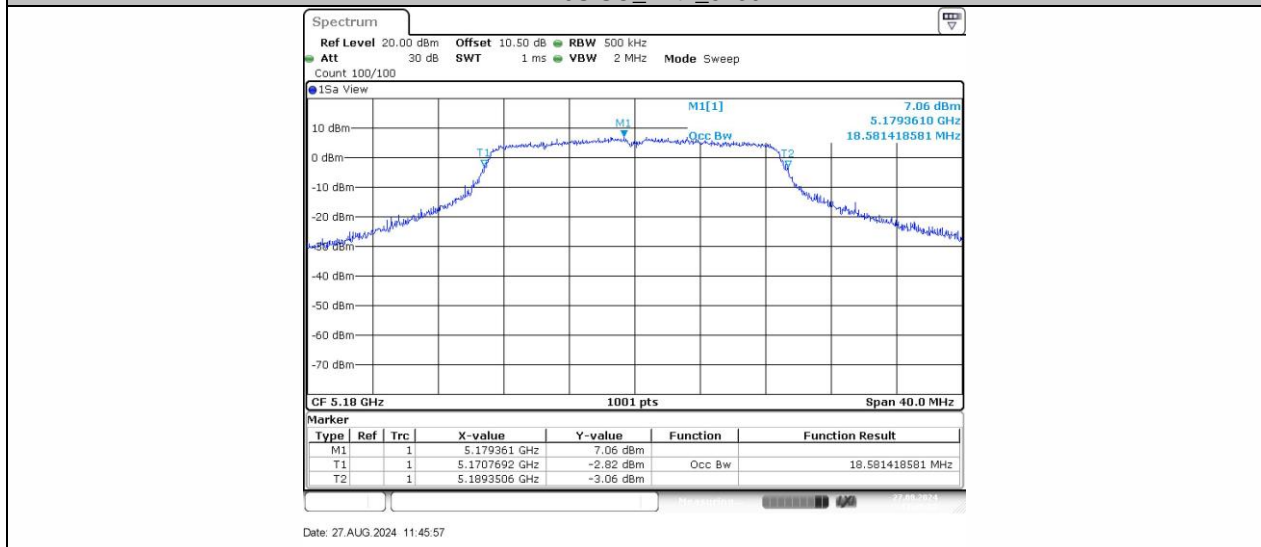
11AC20SISO_Ant1_5180
