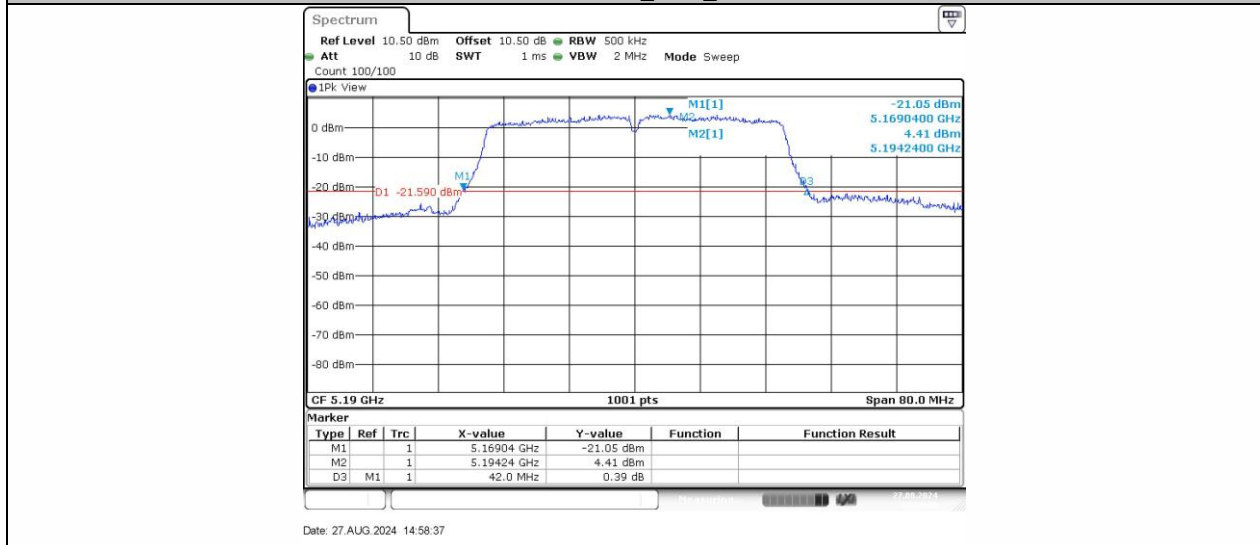
11AC40SISO_Ant1_5190
