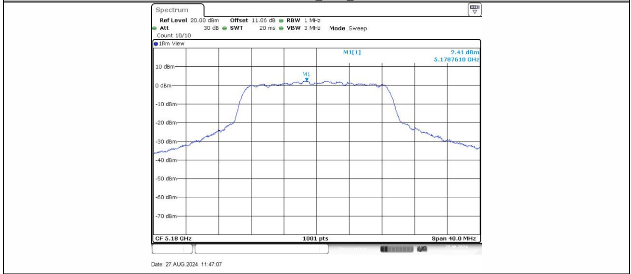
11AC20SISO_Ant1_5180
