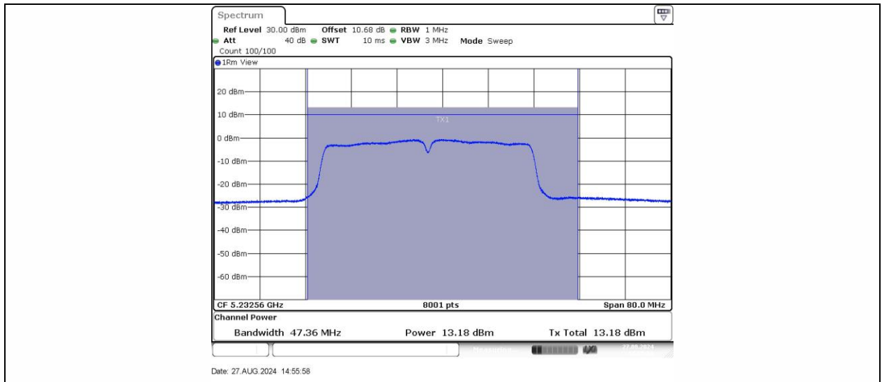
11AC40SISO_Ant1_5230
