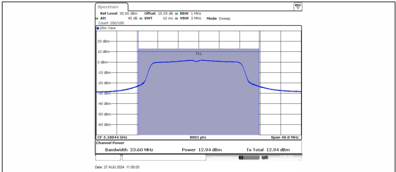
11N20SISO_Ant1_5180
