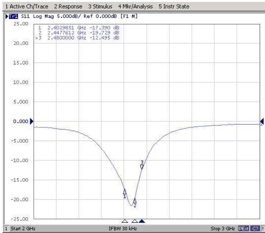
S11
