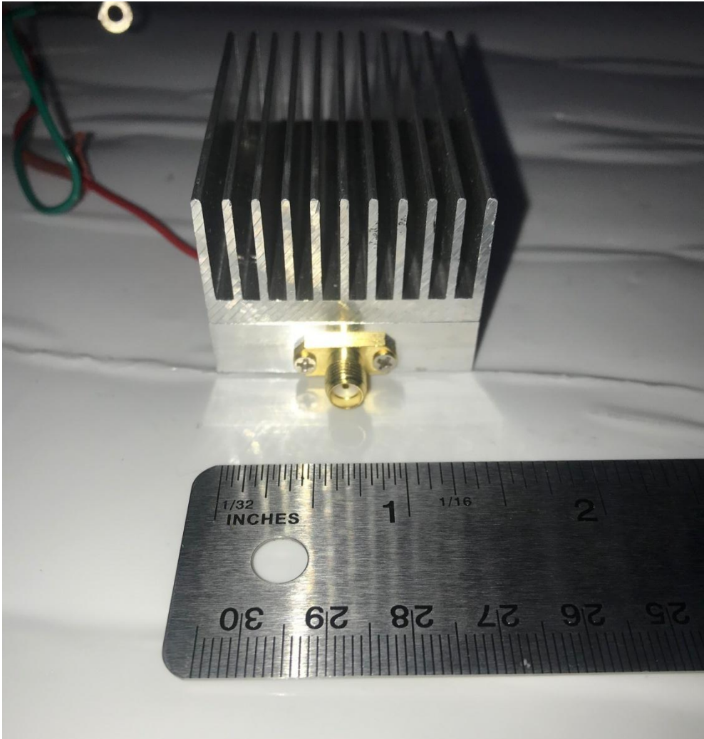
Figure 7. SAFE-1001 (UHF Amp) Top
