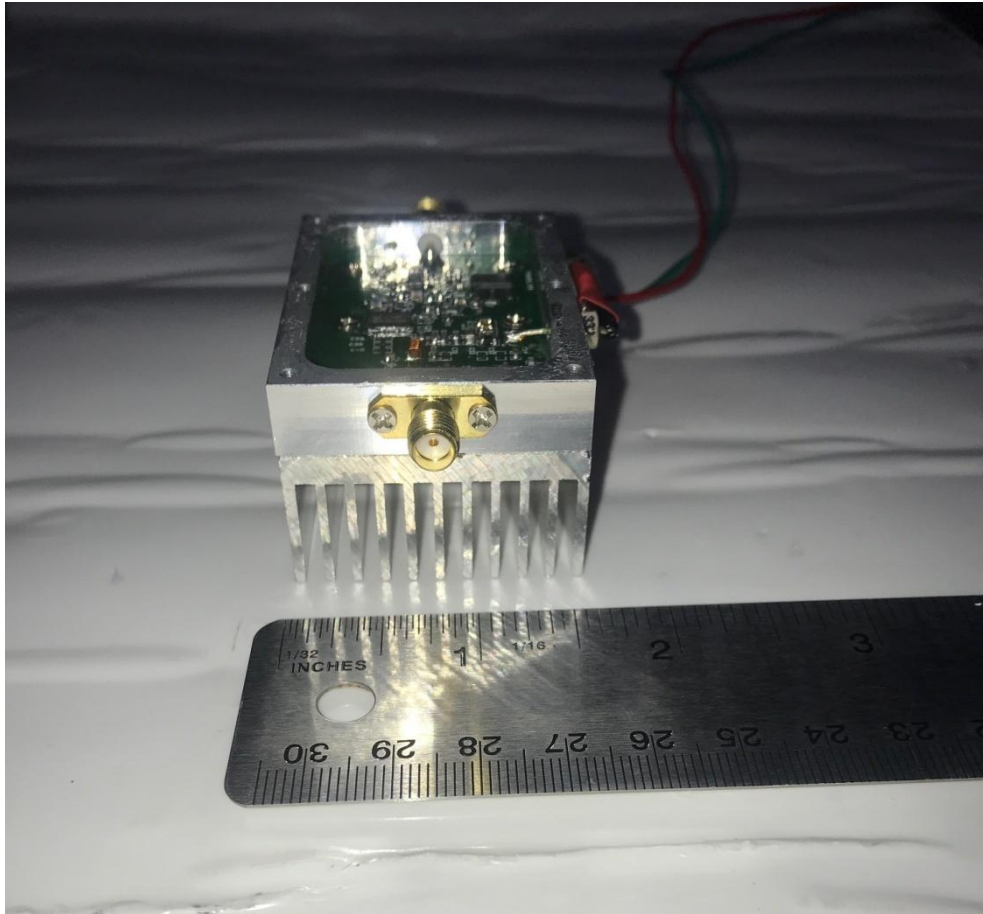
Figure 14. SAFE-1001 (VHF Amp) Bottom
