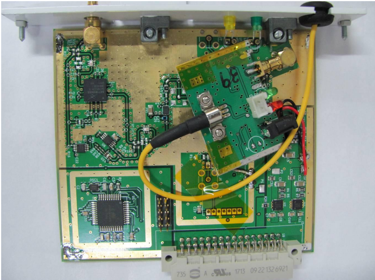
Figure 8. RDL 2.4 (UHF), Shield Removed
