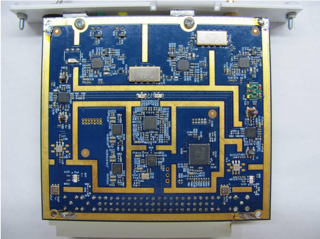
Figure 3. 700 MHz Channel Card, Shield Removed
