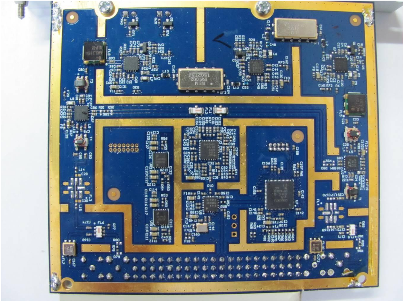
Figure 1. VHF Channel Card, Shield Removed
