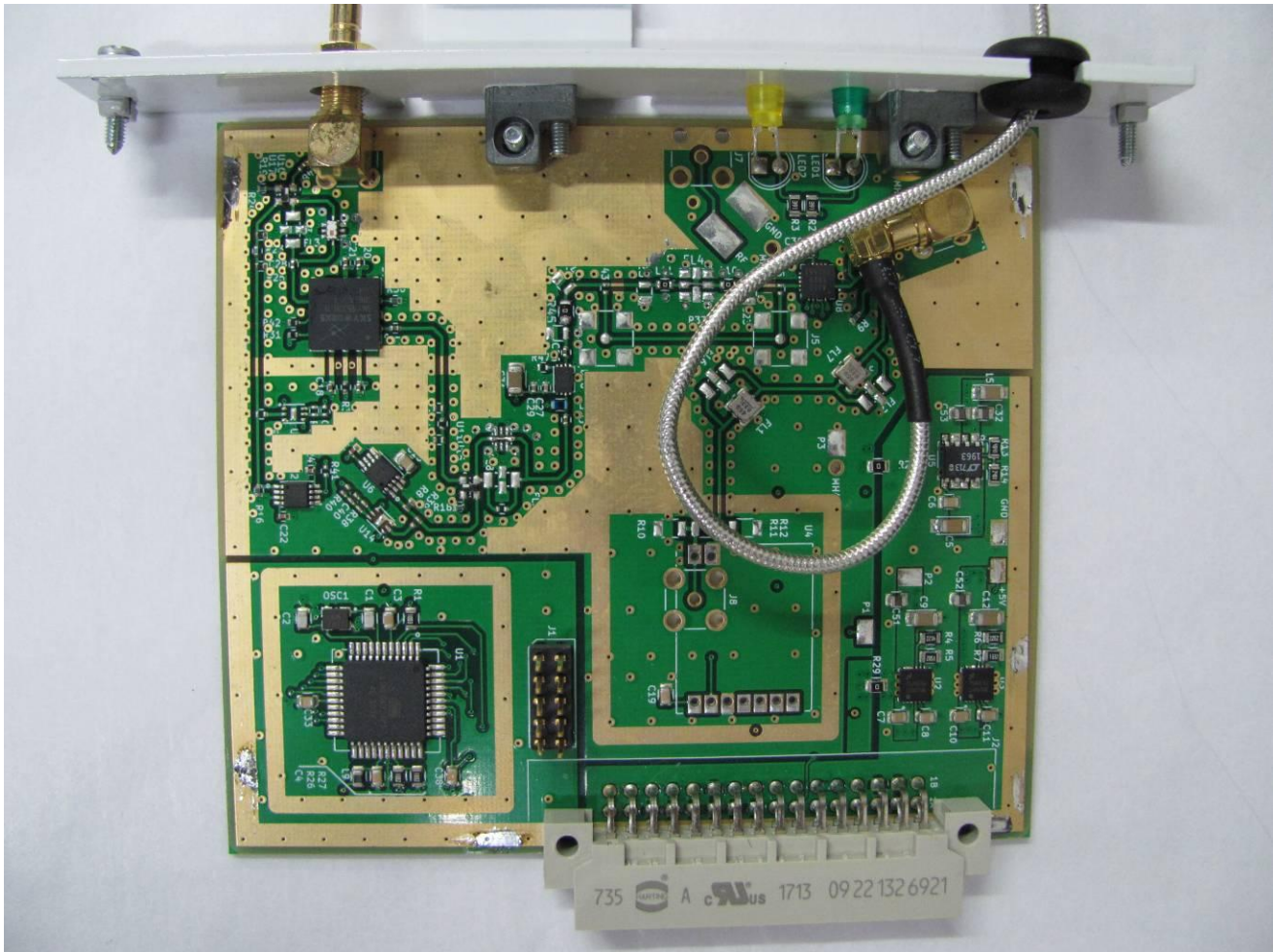
Figure 6. UHF Power Amp, Shield Removed
