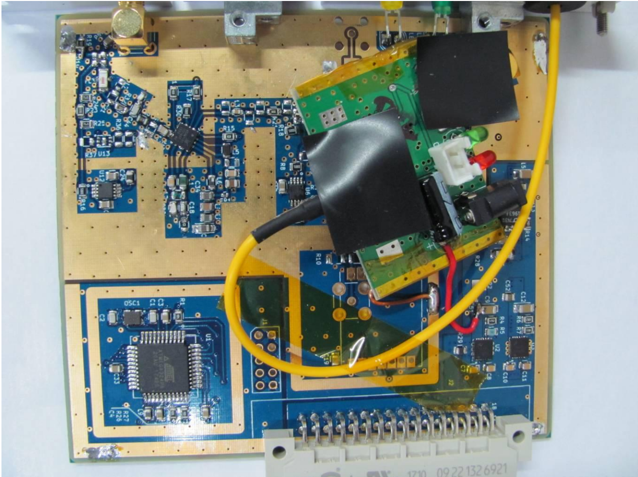
Figure 7. RDL 2.3 (VHF), Shield Removed
