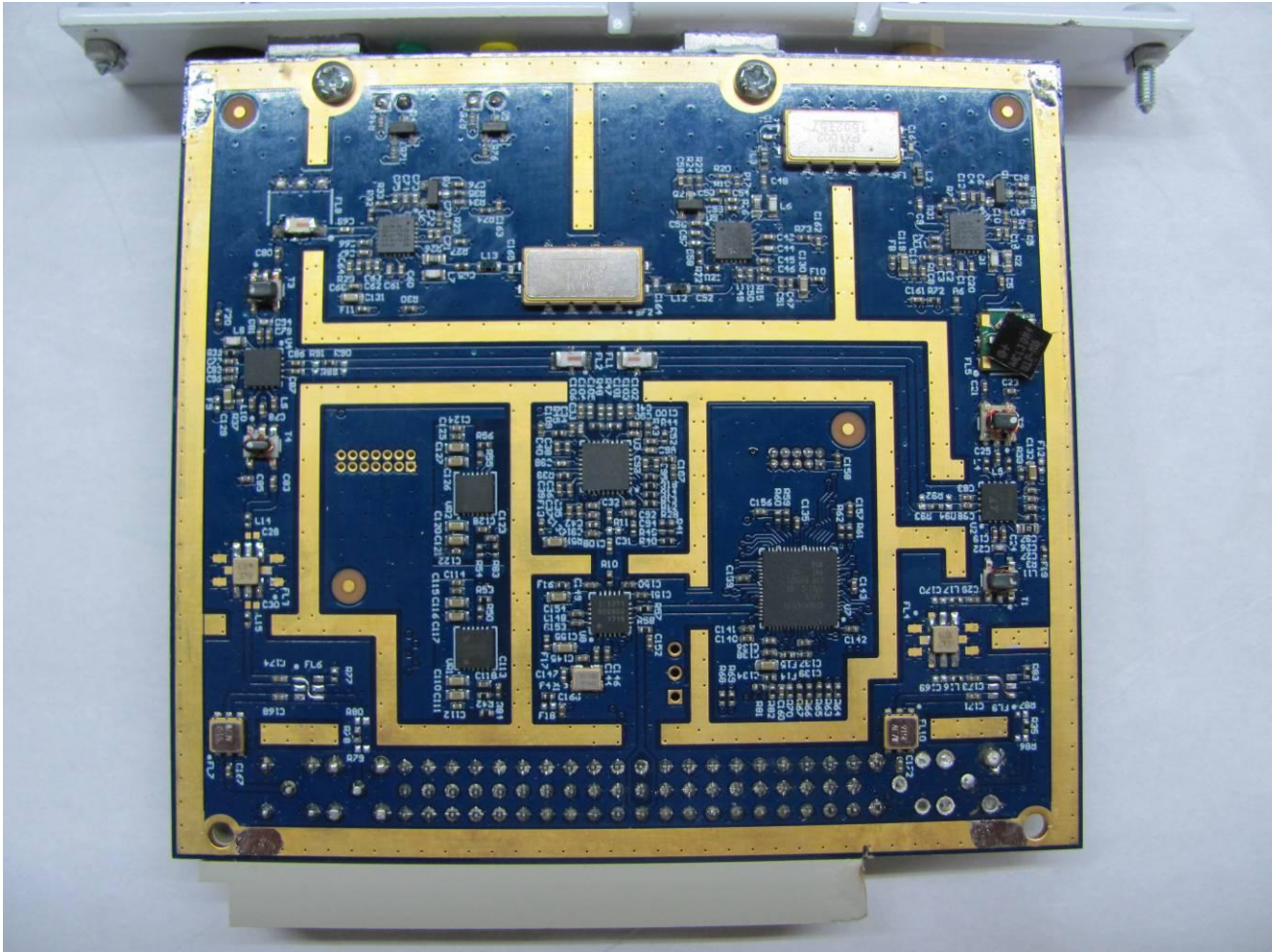
Figure 4. 800 MHz Channel Card, Shield Removed
