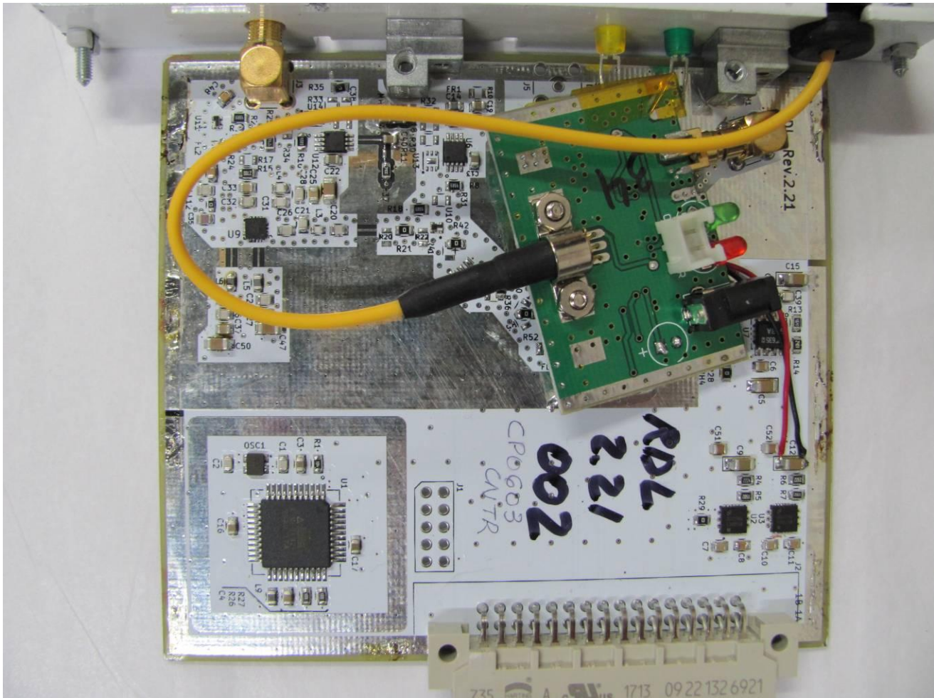
Figure 9. RDL 2.2 (700-900 MHz), Shield Removed
