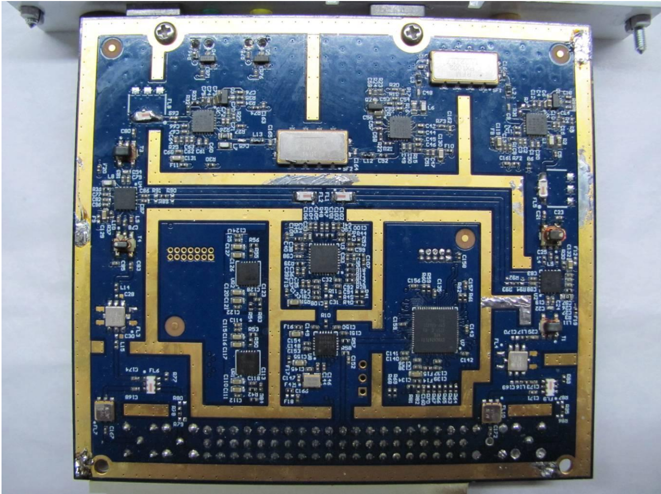
Figure 5. 900 MHz Channel Card, Shield Removed
