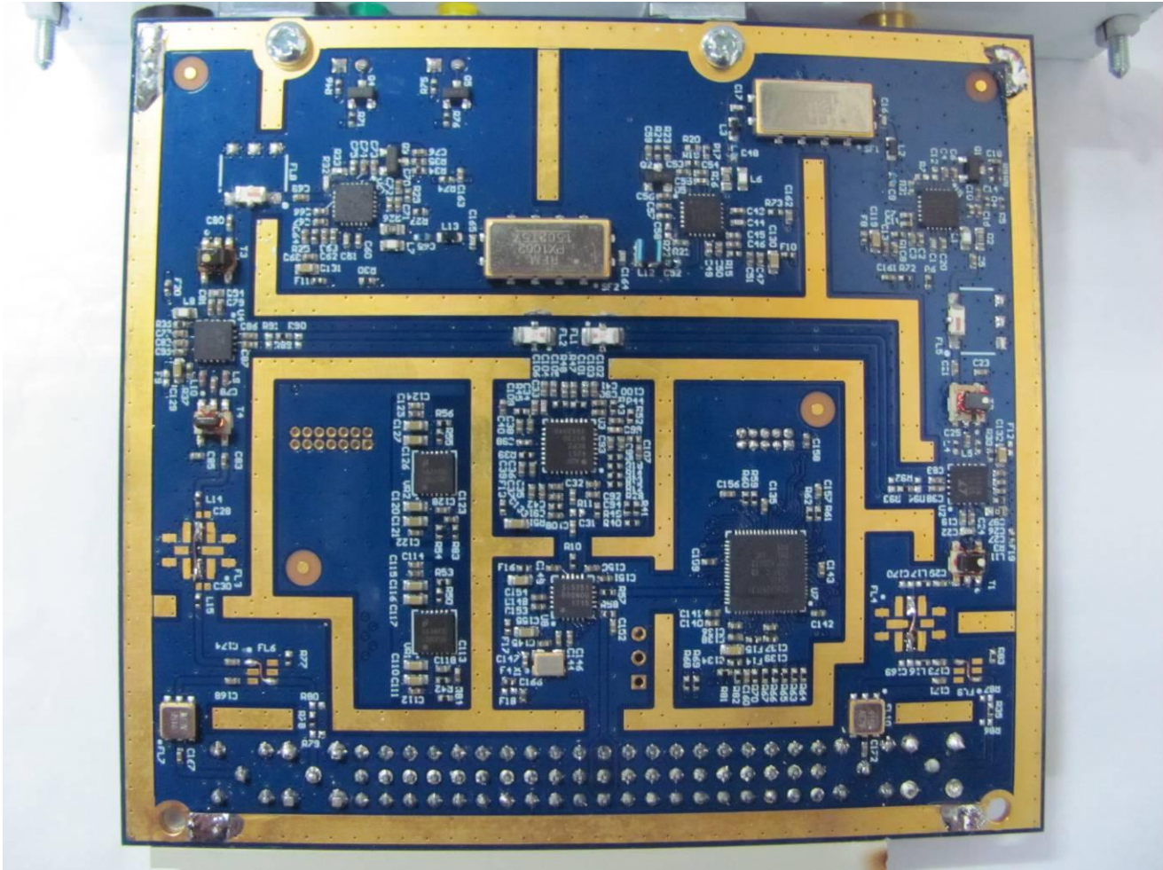
Figure 2. UHF Channel Card, Shield Removed
