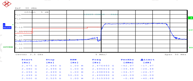
(Channel Bandwidth:20 MHz)_LCH_QPSK_100RB#0
