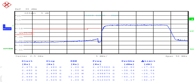
(Channel Bandwidth:20 MHz)_LCH_16QAM_100RB#0
