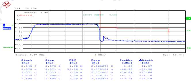
(Channel Bandwidth:20 MHz)_HCH_QPSK_100RB#0
