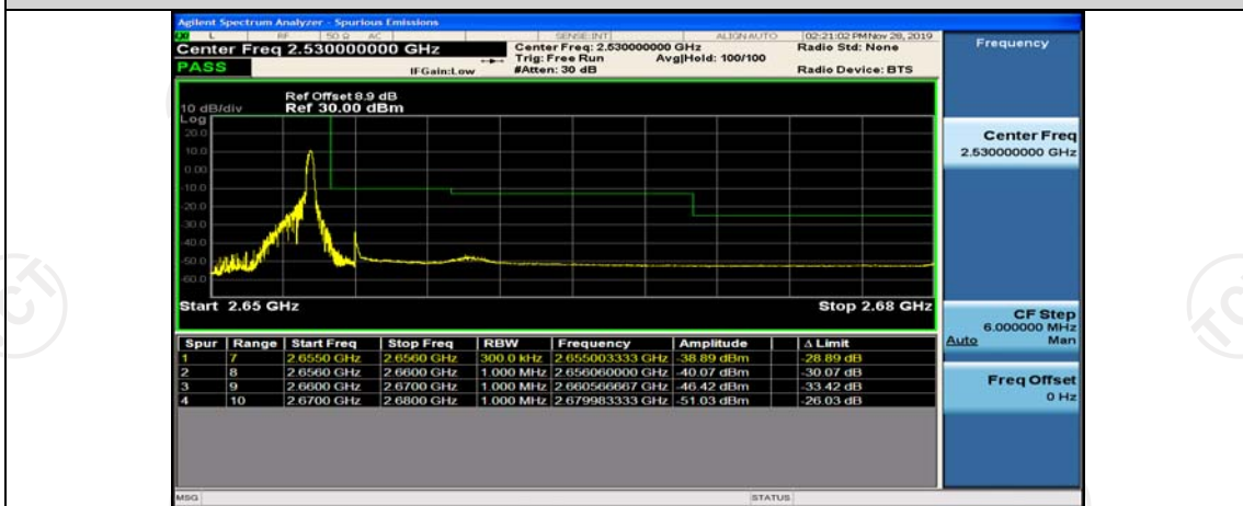
Band41-15MHz-QPSK-41165-75RB#0
