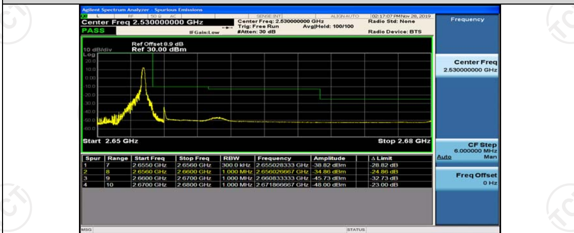
Band41-15MHz-16QAM-41165-1RB#74
