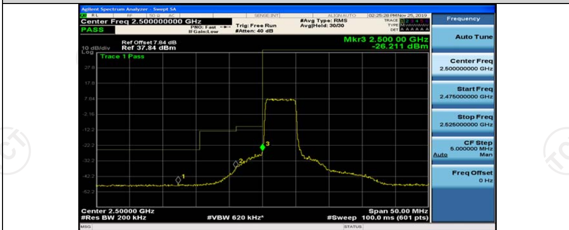
Band7-10MHz-16QAM-20800-25RB#25
