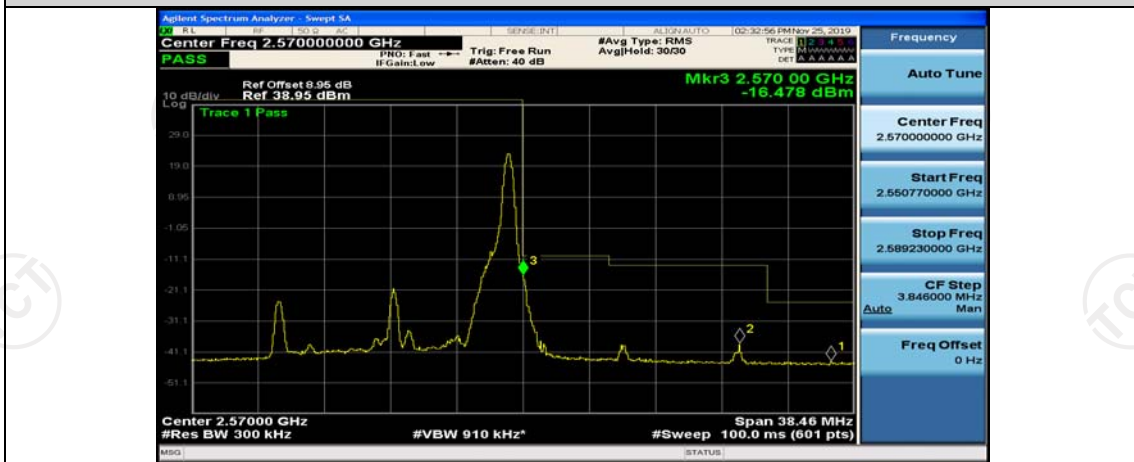
Band7-15MHz-16QAM-21375-38RB#0
