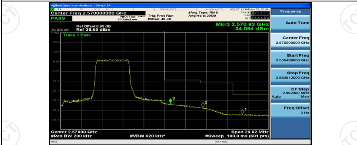
Band7-10MHz-QPSK-21400-50RB#0
