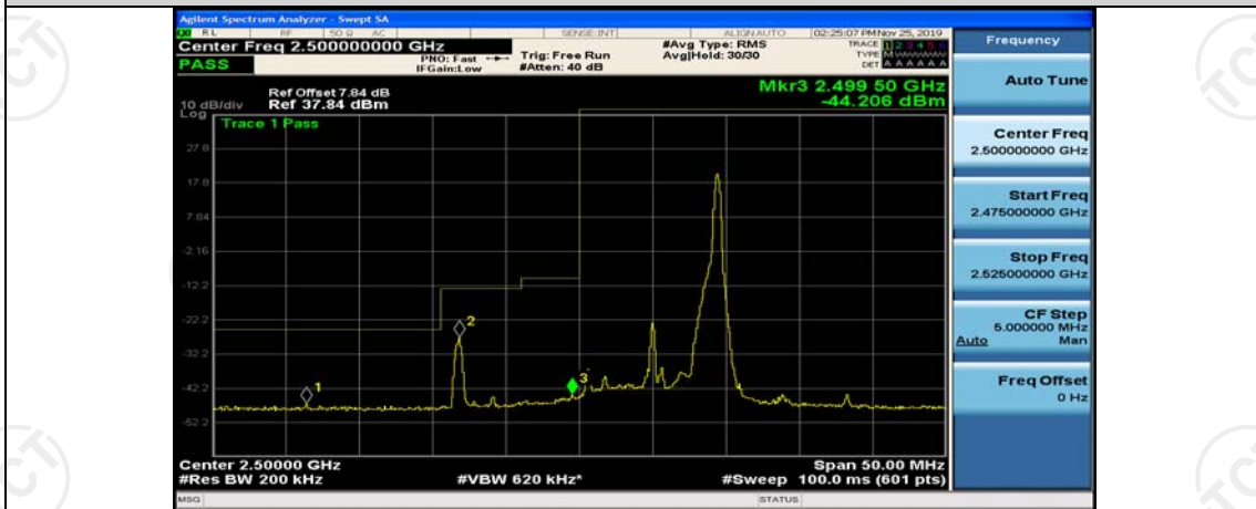
Band7-10MHz-16QAM-20800-25RB#0
