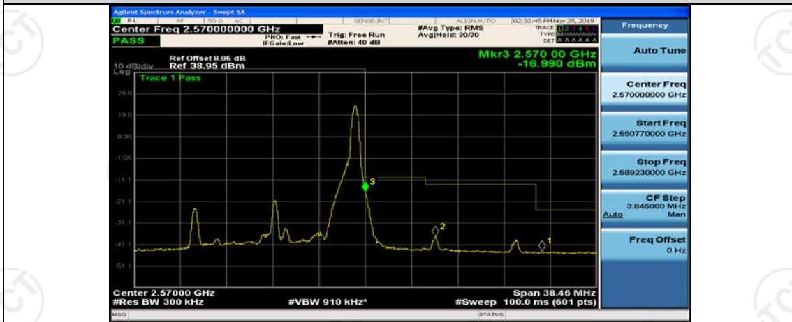
Band7-15MHz-QPSK-21375-38RB#0
