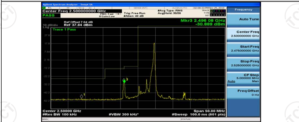
Band7-5MHz-16QAM-20775-1RB#0
