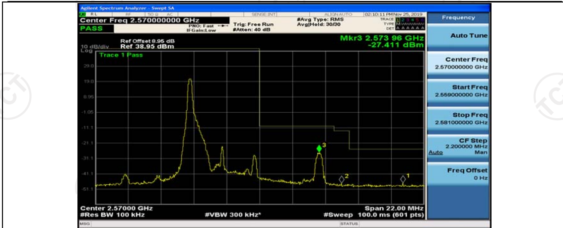
Band7-5MHz-16QAM-21425-1RB#24
