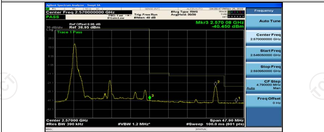
Band7-20MHz-QPSK-21350-1RB#99
