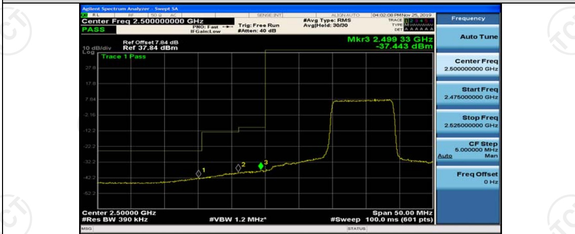
Band7-20MHz-16QAM-20850-100RB#0
