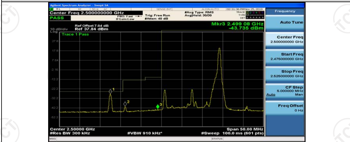
Band7-15MHz-16QAM-20825-38RB#0
