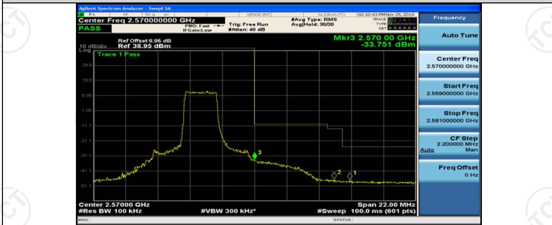
Band7-5MHz-QPSK-21425-12RB#13
