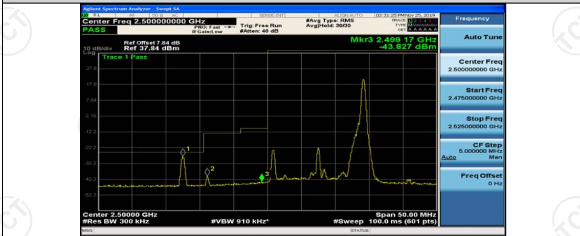
Band7-15MHz-QPSK-20825-75RB#0
