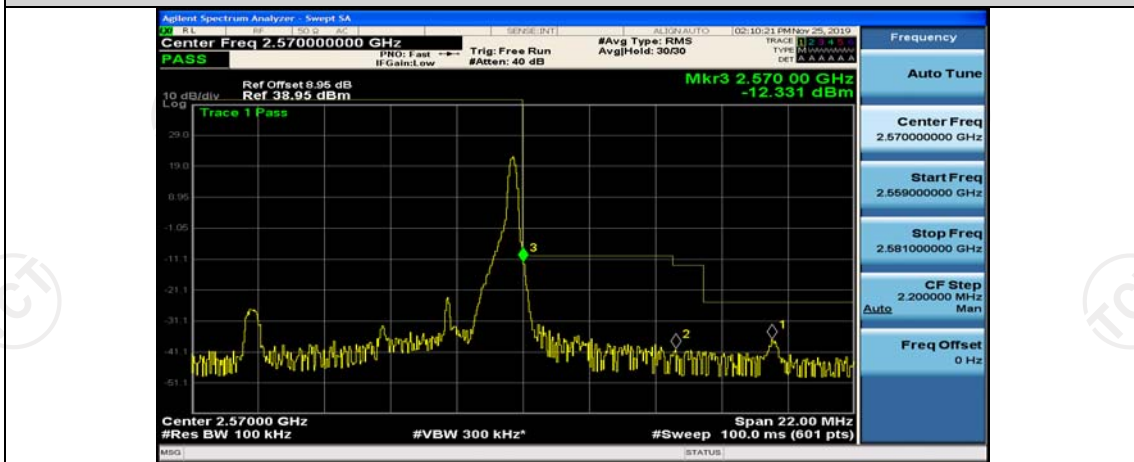
Band7-5MHz-QPSK-21425-1RB#0
