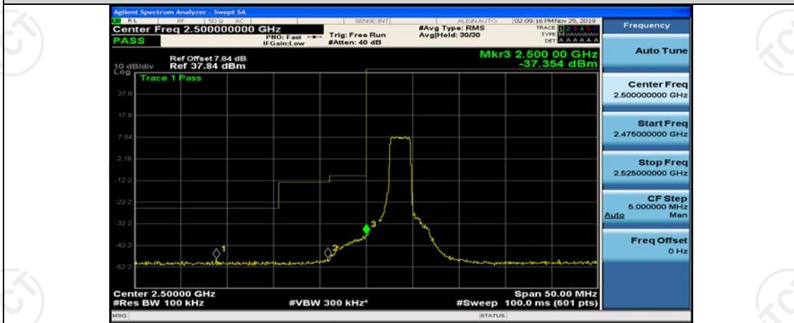
Band7-5MHz-16QAM-20775-25RB#0
