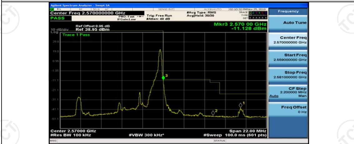
Band7-5MHz-16QAM-21425-12RB#0
