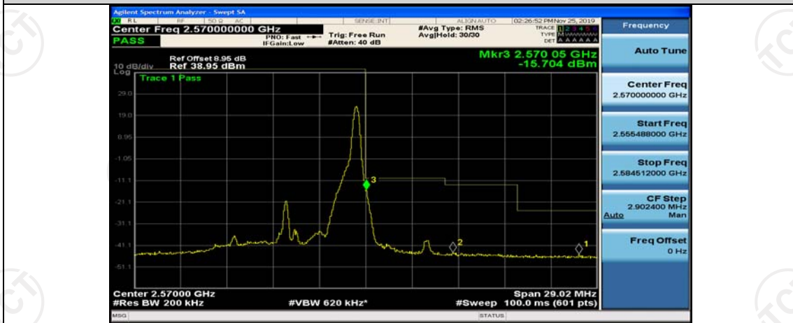
Band7-10MHz-QPSK-21400-1RB#0
