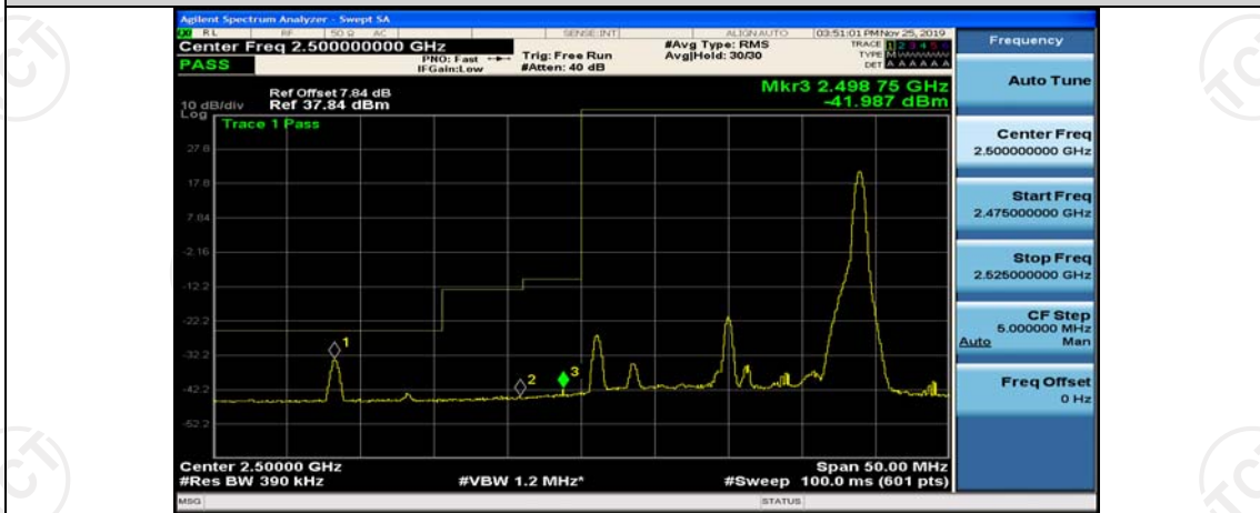
Band7-20MHz-QPSK-20850-50RB#50
