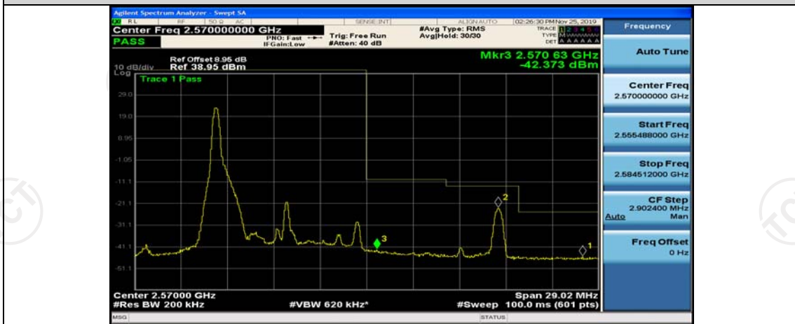
Band7-10MHz-QPSK-21400-25RB#25
