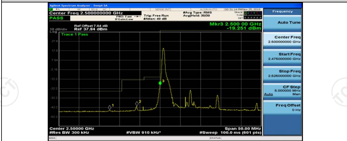
Band7-15MHz-16QAM-20825-75RB#0
