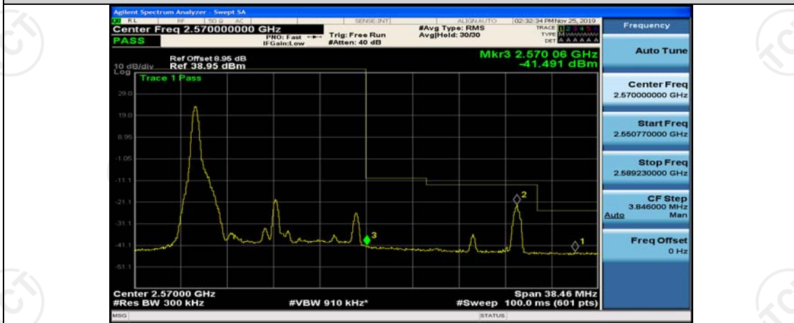
Band7-15MHz-16QAM-21375-1RB#74
