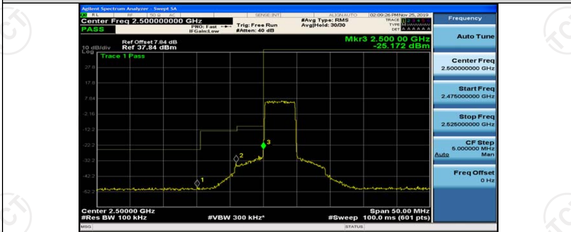
Band7-5MHz-QPSK-212425-1RB#24
