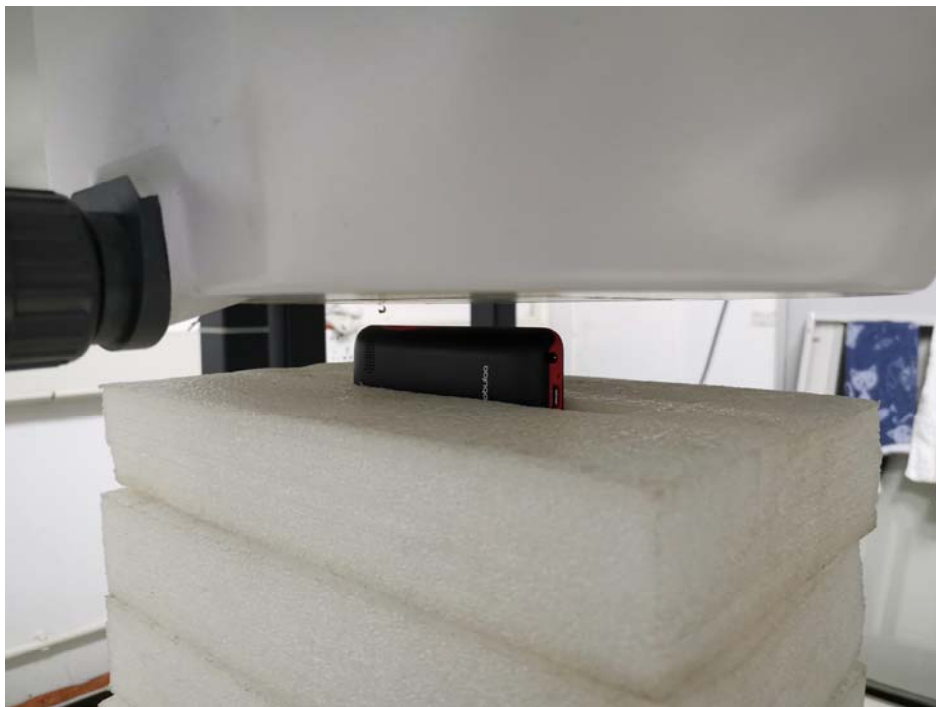
Body worn – Left (10mm)
