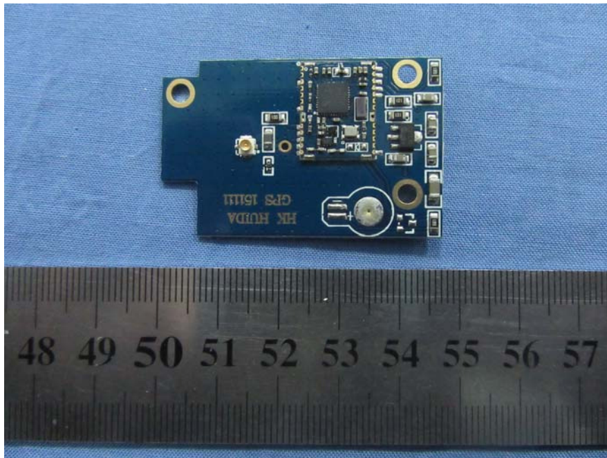
EUT –GPS Board Uncover View
