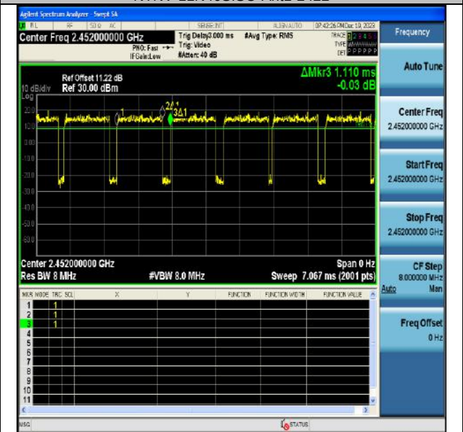
NTVN-11N40SISO-Ant1-2452
