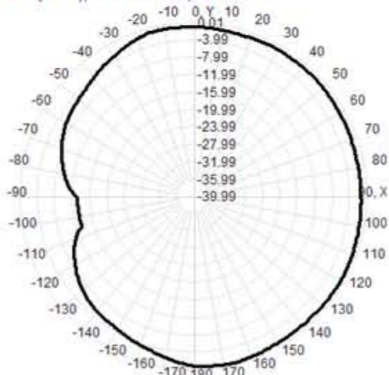
Total(H-XY), Max= -0.70dBi, CirD=12.73
