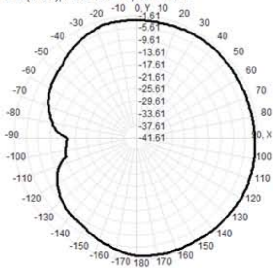
Total(H-XY), Max= -2.05dBi, CirD=17.22
