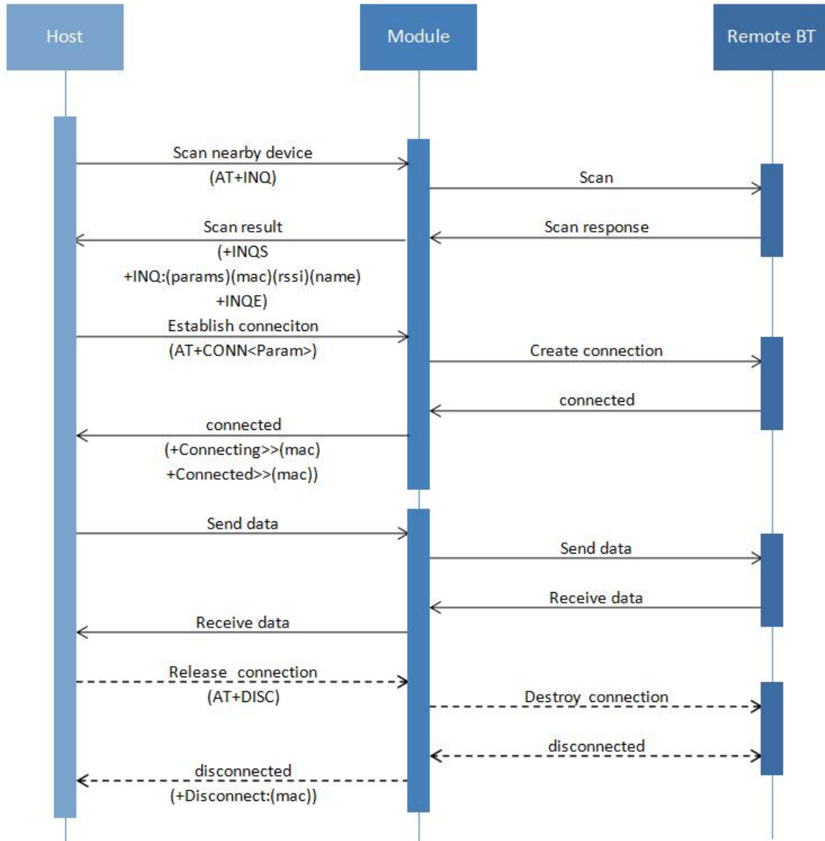
Figure 8: Master-slave module communication flow chart
