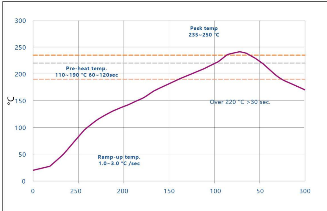
Figure 19: Recommended reflow soldering temperature profile
