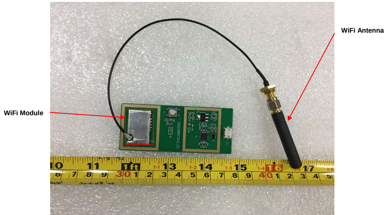
EUT Attached in Test Board View
