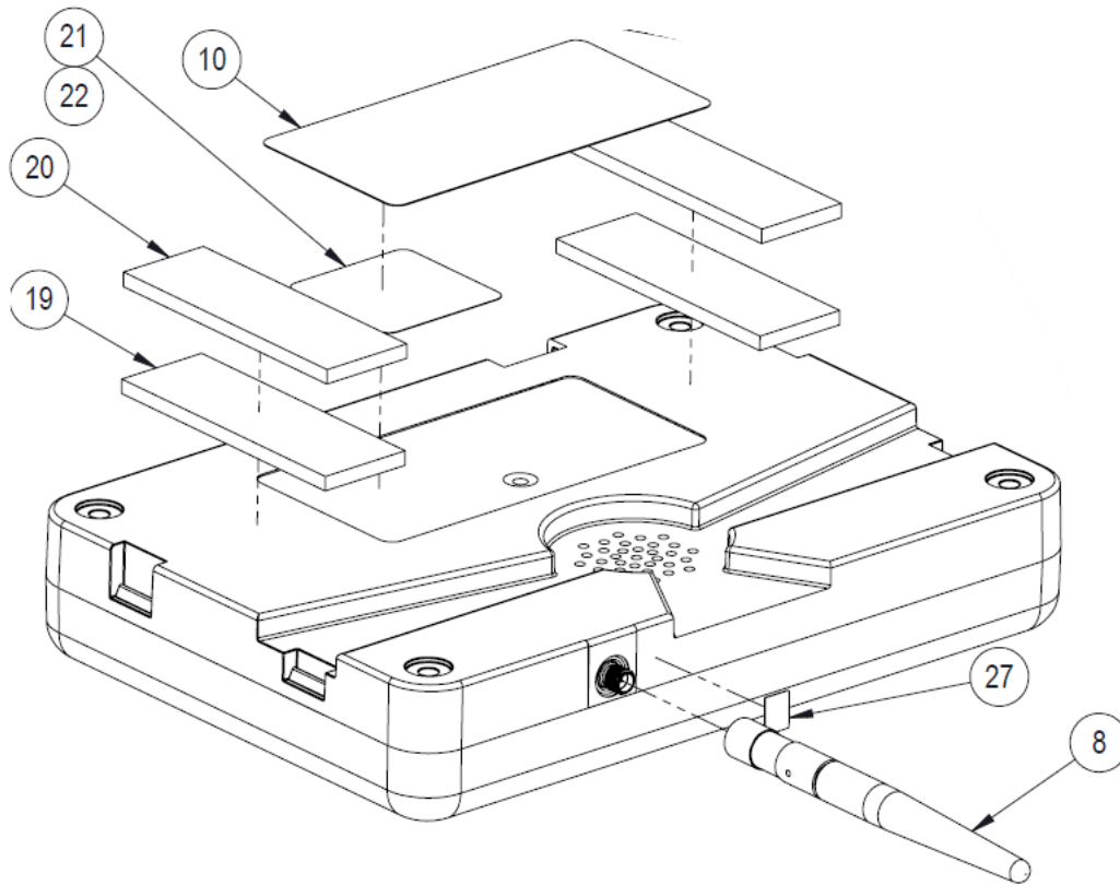
Figure 4. Placement of labels (Items #10 and #21) on rear panel of 3665 RALU Display Module.
