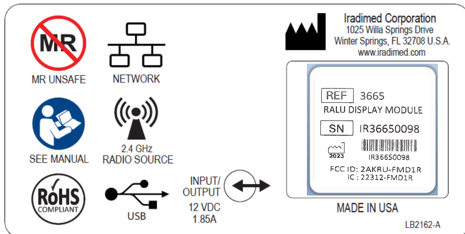
Figure 3. RALU Display Module identification label (Item #21) placed in window of LB2162 information label (Item #10).
