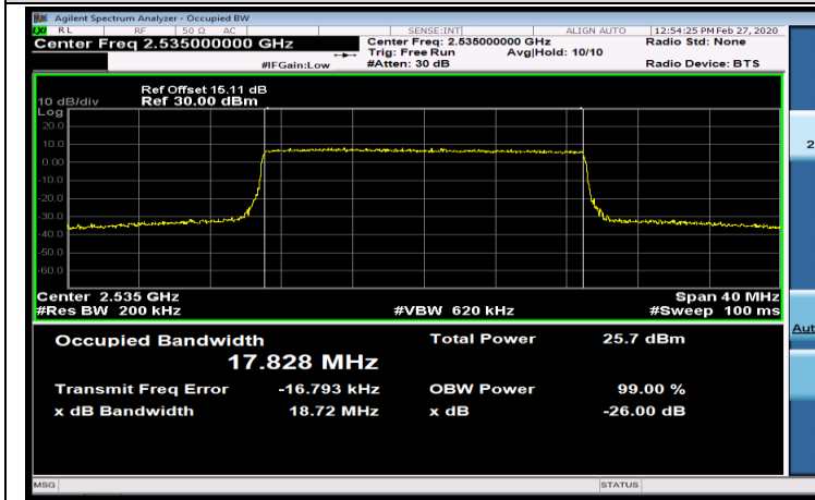
MCH_QPSK_100RB#0
