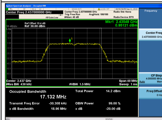
802.11g 99% Bandwidth - Mid CH 2437
