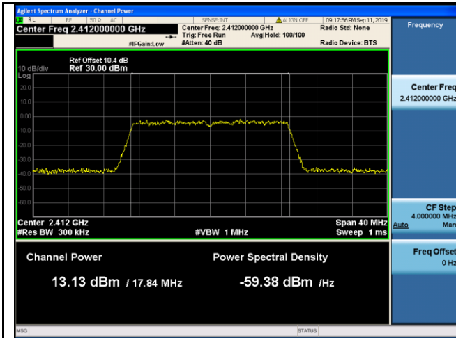
802.11n20 - Maximum Output Power - Low CH 2412
