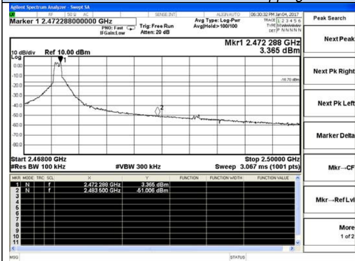
Channel 15 / 2472 MHz – Non-Hopping
