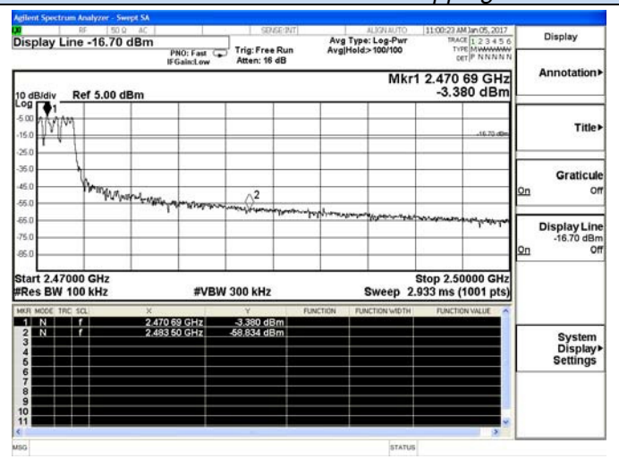
Channel 15 / 2472 MHz – Hopping
