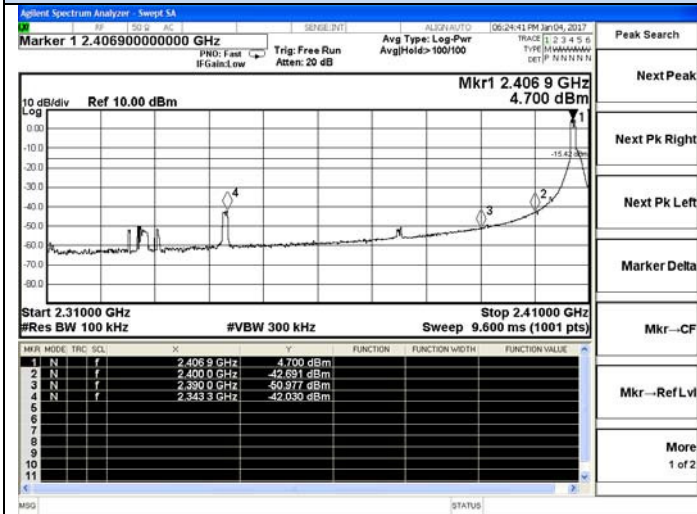
Channel 0 / 2407 MHz – Non-Hopping
