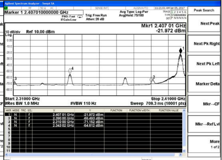
Channel 0 / 2407 MHz-Average
