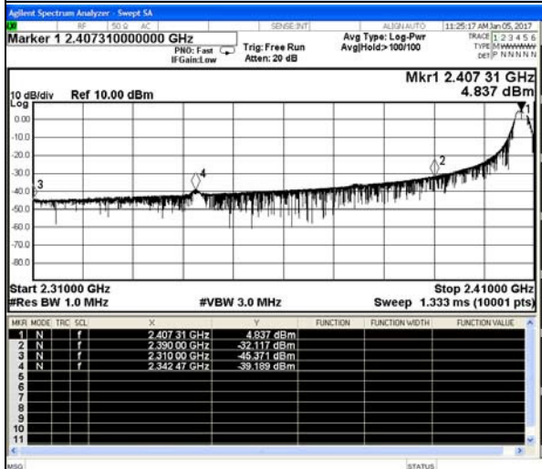
Channel 0 / 2407 MHz- Peak
