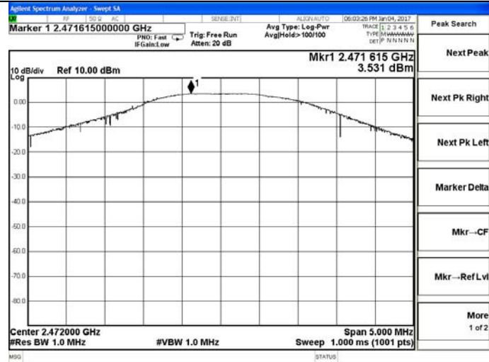
Channel 15/ 2472 MHz
