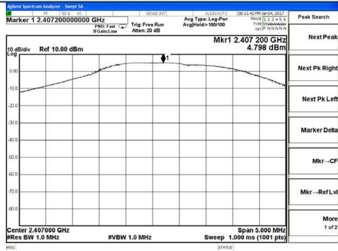
Channel 0 / 2407 MHz
