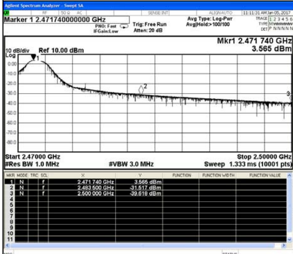
Channel 16 / 2472 MHz- Peak
