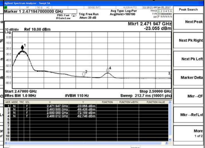
Channel 16 / 2472 MHz-Average
