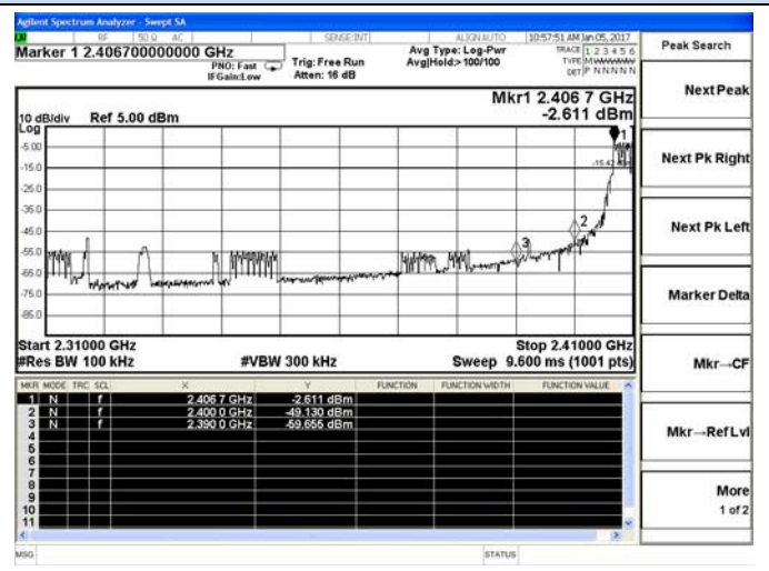
Channel 0 / 2407 MHz – Hopping
