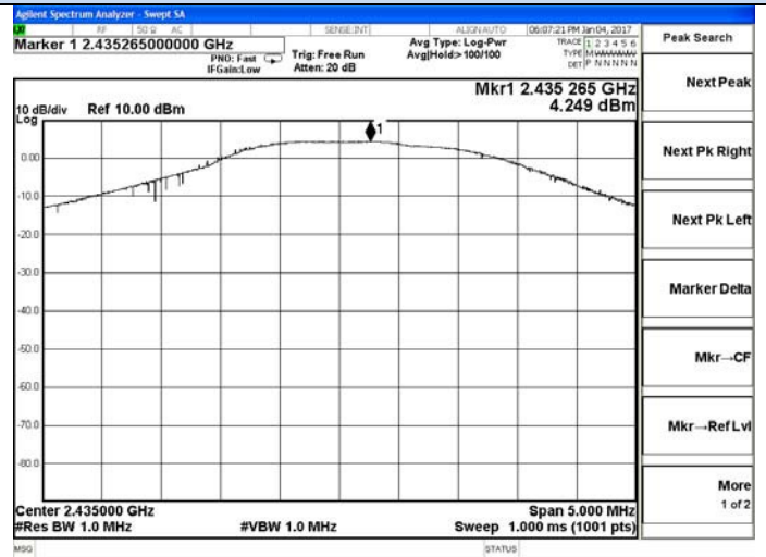
Channel 5 / 2435 MHz
