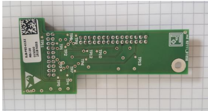
ELB-PED-0132-00 Paradox Crypto Engine board
