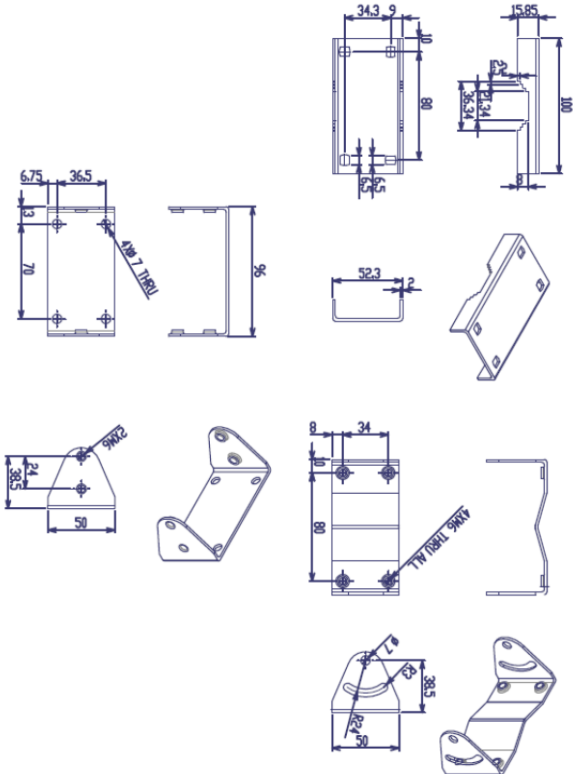
Figure 10 Dimensions of the mounting brackets
