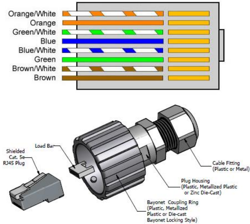
Figure 8 Pinout of the Ethernet connector and IP67 Ethernet connector
