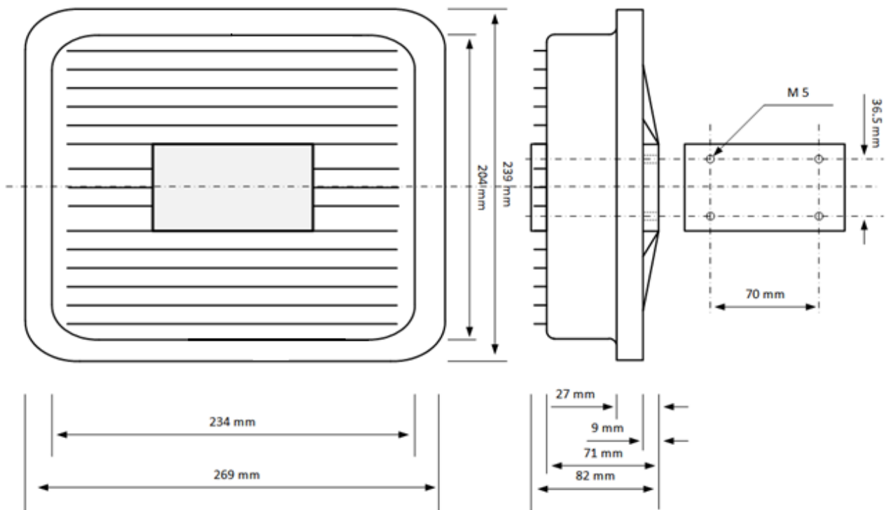
Figure 9 Dimensions of the Gateway
