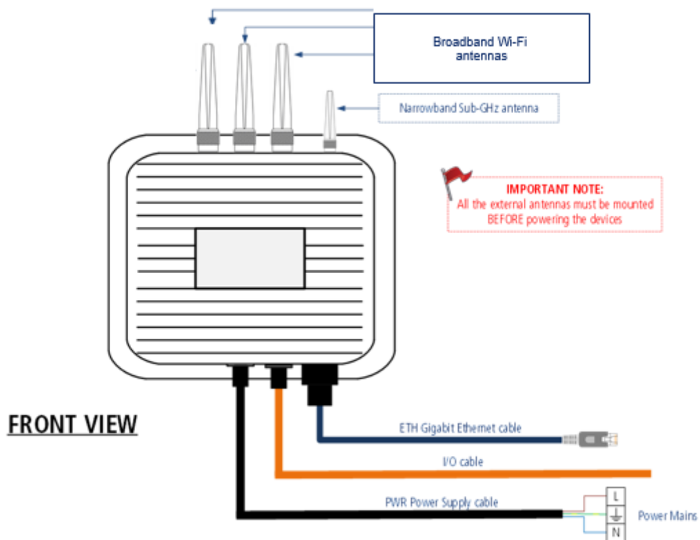
Figure 5 Wiring scheme for the installation of the Gateway.
