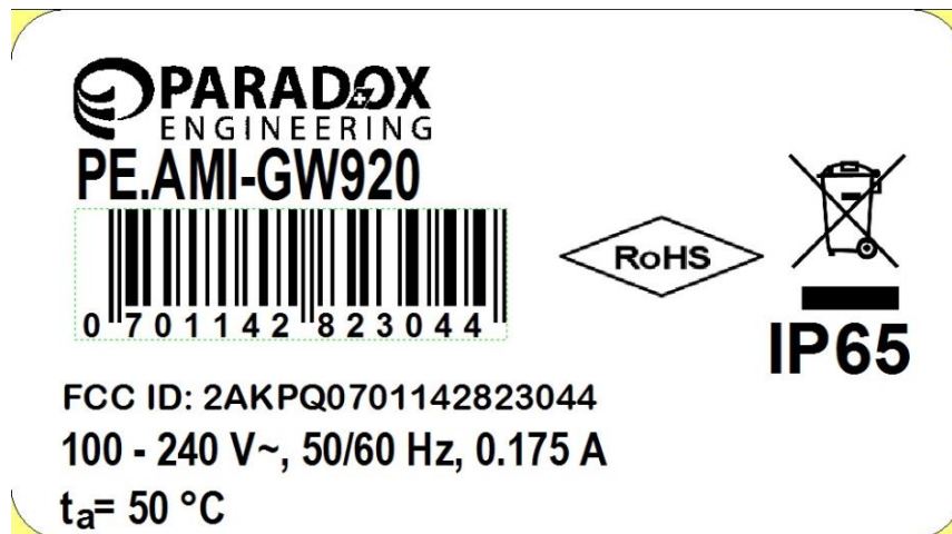
Figure 11 Label of the PE.AMI-GW
