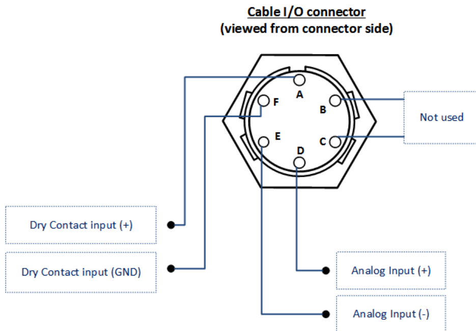
Figure 7 Scheme of the pinout of the I/O connector, as viewed from the connector side.
