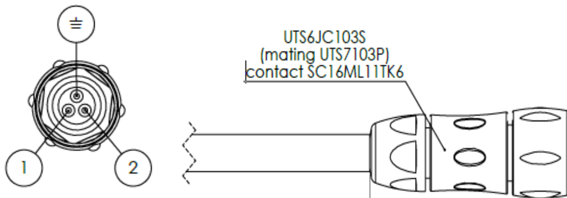
Figure 6 Scheme of the pinout of the power cable, as viewed from the connector side.
