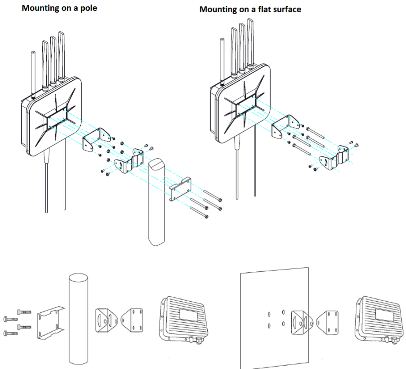
Figure 2 Instructions for mounting PE.AMI Gateway on a pole (left side) and on a flat surface (right side).
