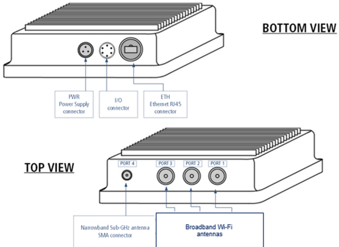
Figure 4 Positions and names of connectors available for the Gateway (top and bottom views).
