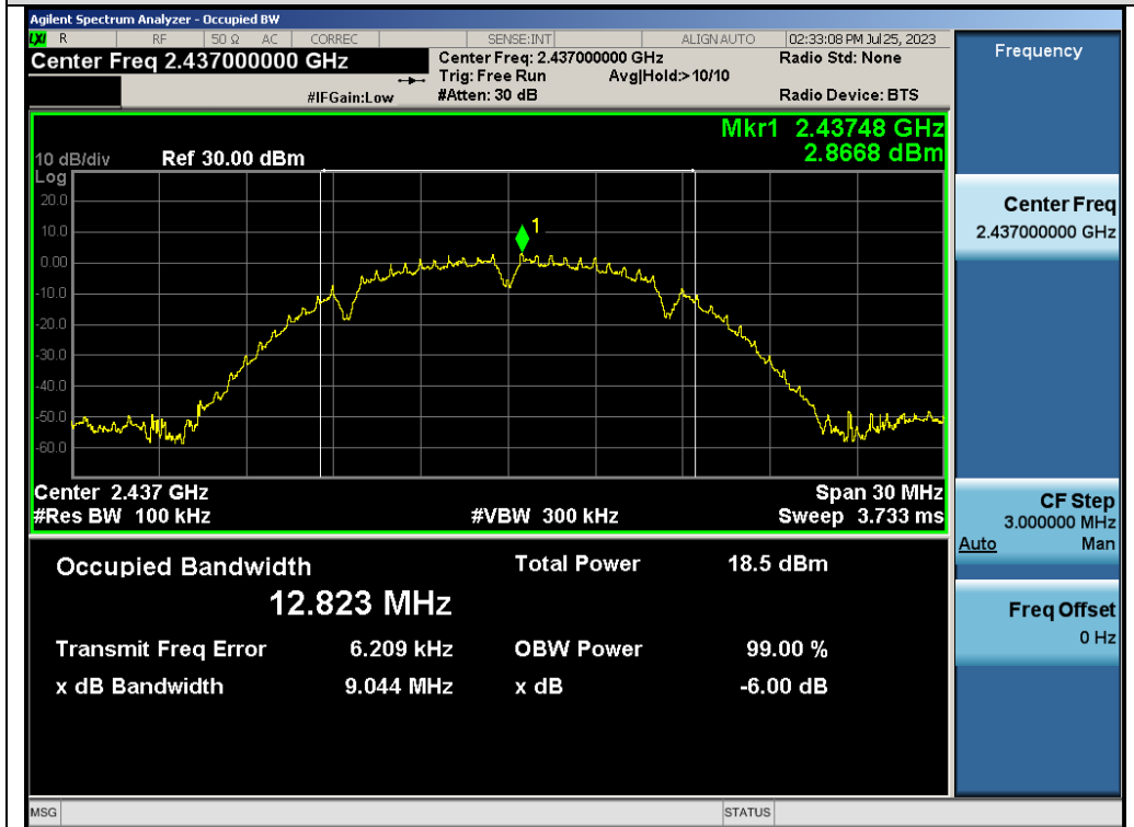
Test_Graph_802.11b_ANT1_2437_1Mbps_DTSBW
