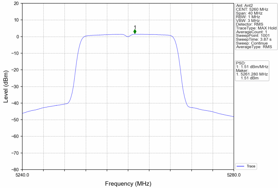
802.11n(HT20)_LCH_5260MHz_MIMO_NTNV
